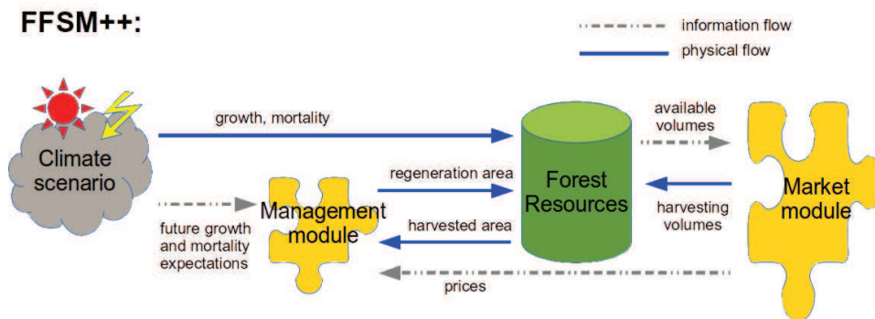
Figure 1: FFSM++ Flowchart
