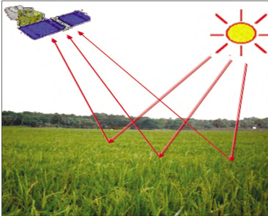
Figure 3. Geometrical configuration in a typical remote sensing system composed of illumination source (Sun), satellite, atmosphere and surface with different features. The geometrical parameters are Sun angle, viewing or observation angle and their relative azimuth angle.
