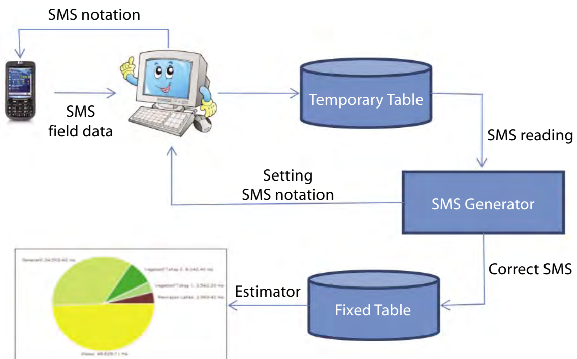
Figure 6. Structure of SMS communication system for AFS
