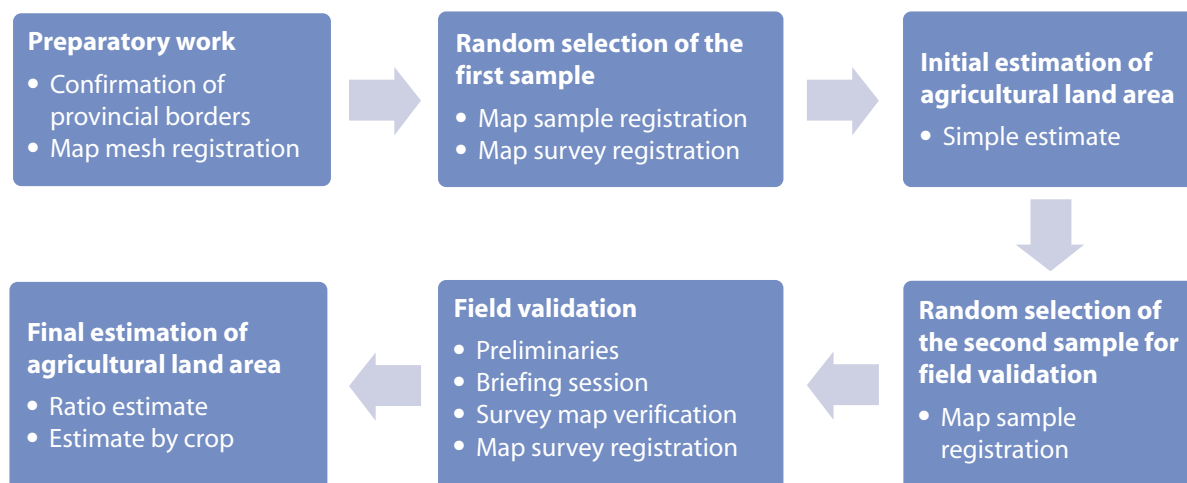
Figure 1. ALIS Workflow
