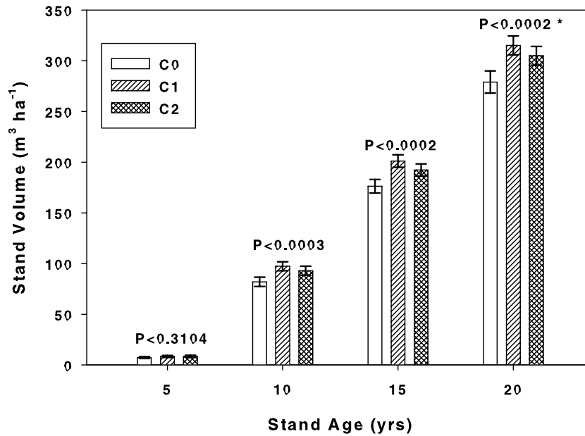
Figure 2—Loblolly pine volume following three levels of compaction [no machine traffic (C0), moderate compaction (C1), and severe compaction (C2)] across 10 blocks of the southern LTSP study in Mississippi, Louisiana, and Texas. *Indicates n=7 because Texas blocks had not reached 20 years old.
