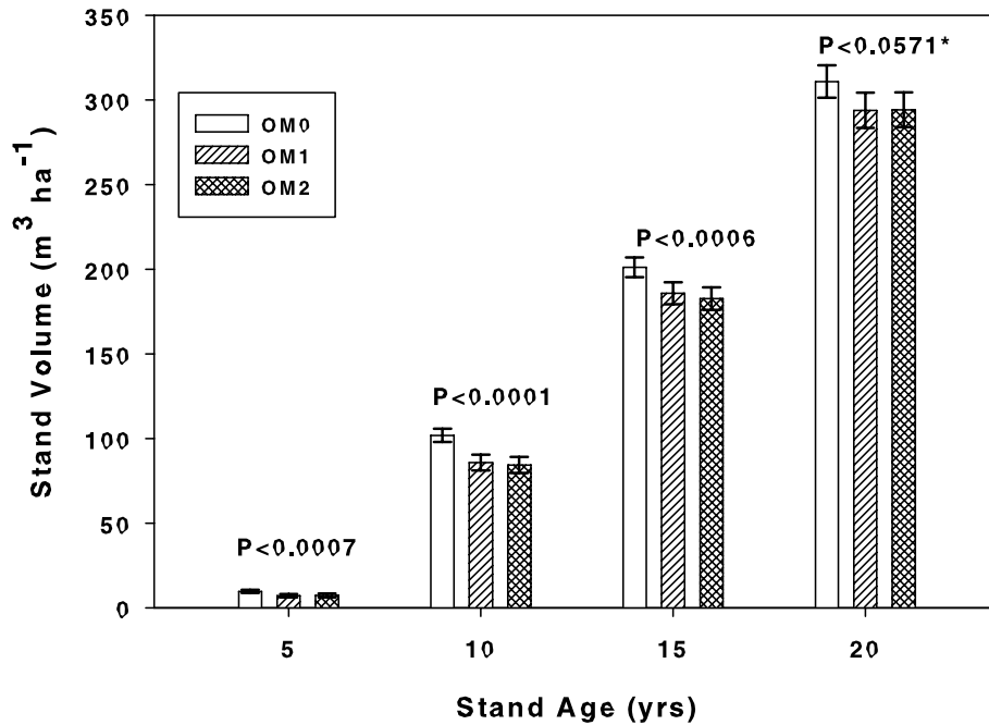
Figure 4—Pine volume following three levels of organic matter removal [bole-only harvest (OM0), whole-tree harvest (OM1), and complete organic matter removal (OM2)] across 10 blocks of the southern LTSP study in Mississippi, Louisiana, and Texas. *Indicates n=7 because Texas blocks had not reached 20 years old.
