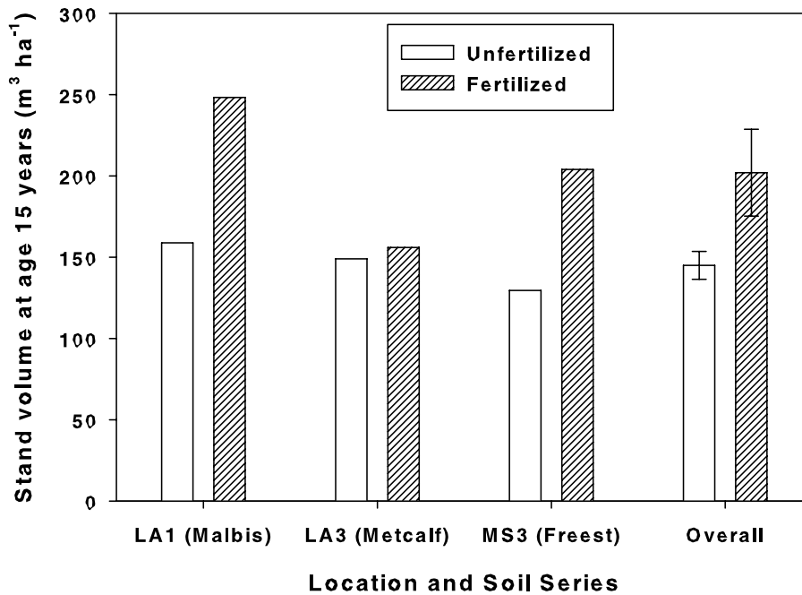
Figure 5—Pine volume response to fertilizer (56 and 44 kg ha⁻¹ of phosphorus and nitrogen, respectively, applied at age 4) on three whole-tree harvested plots with operational compaction at age 15 (see table 1 for location information).
