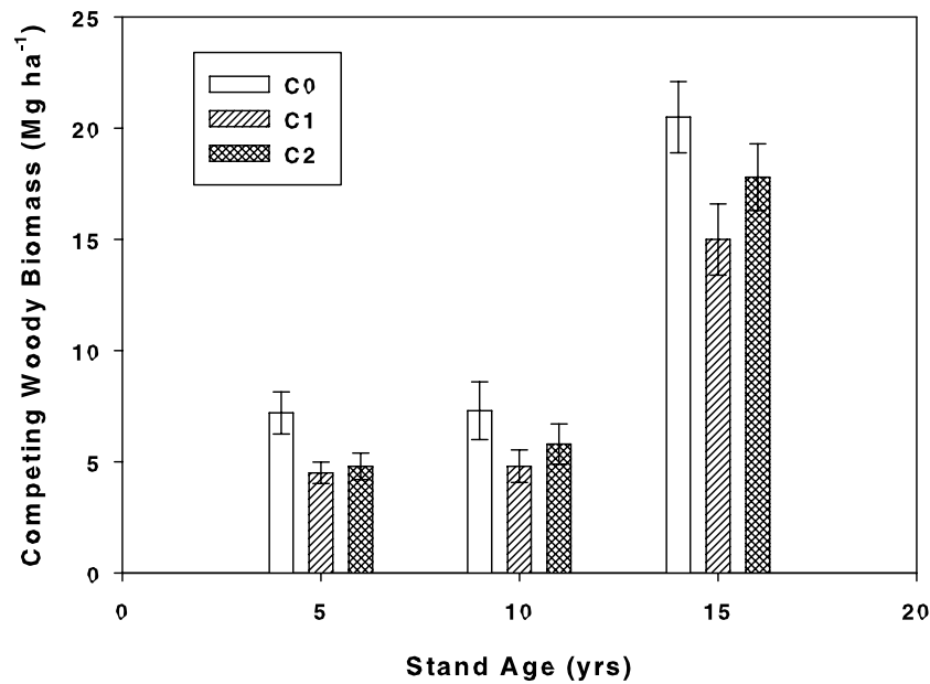
Figure 3—Biomass of competing woody vegetation following three levels of compaction [no machine traffic (C0), moderate compaction (C1), and severe compaction (C2)] across 10 blocks of the southern LTSP study in Mississippi, Louisiana, and Texas.
