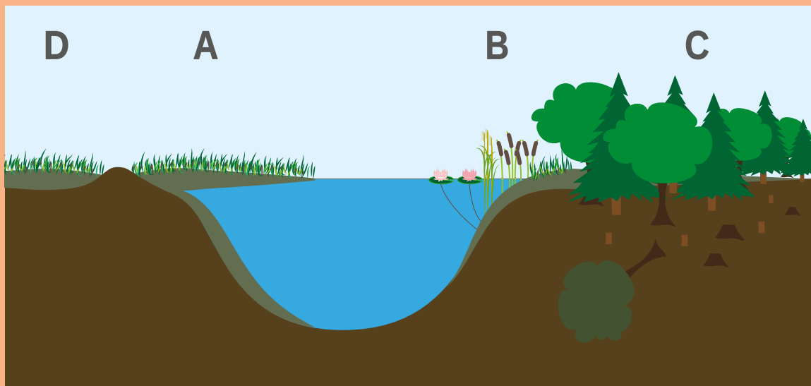
Figure 3.3 Schematic display of a mire formation (modified after Eurola, 1999).
