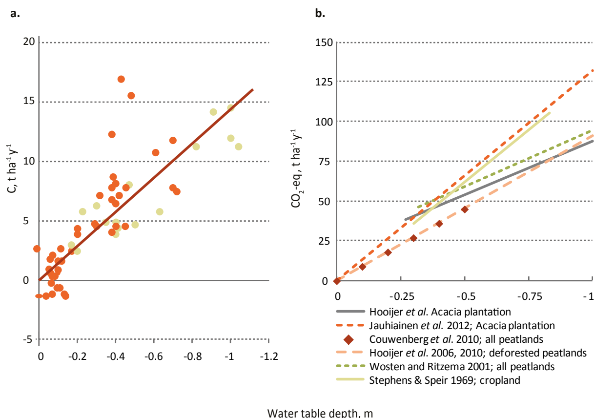
Figure 6.1 Relations between water table depth and CO 2 emission (more than 5 years after drainage) for temperate/boreal and tropical peatlands that have been drained and managed for croplands and plantations (a: from Couwenberg and Hooijer, 2013, b: from Hooijer et al. , 2012). Note that recent research indicates that emissions from non-agricultural peatlands are lower even at the same water table depth.
