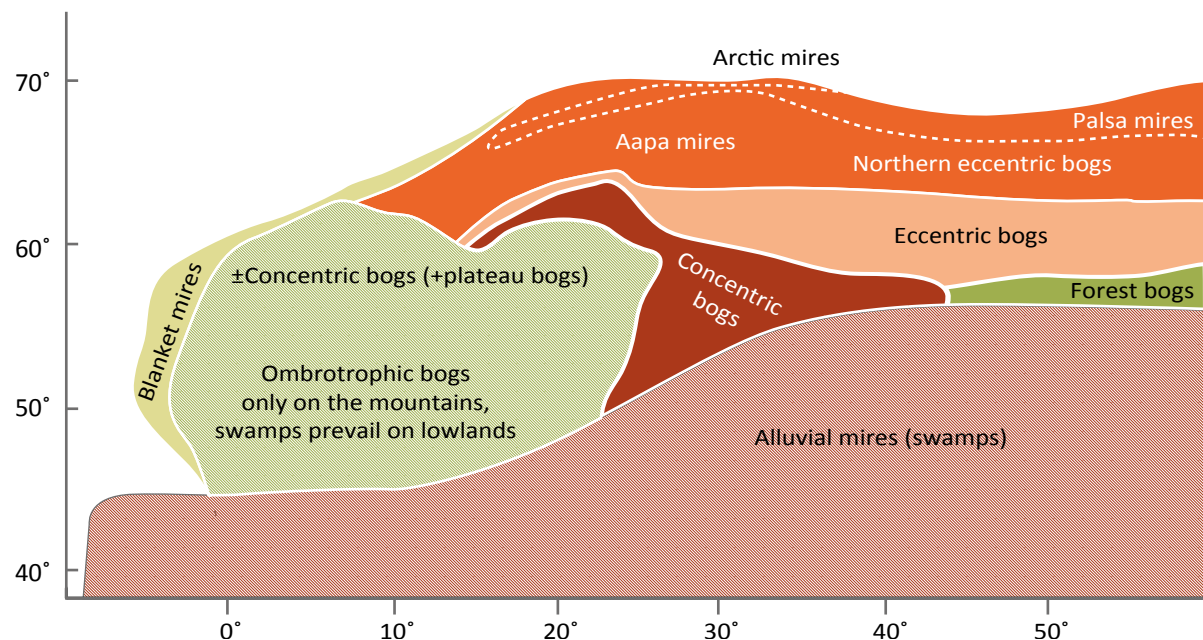
Figure 3.2 The mire regions of Europe. The schematic map, excludes shelf-seas, bays, enclosed seas, etc. The x and y axes present geographic coordinates. Modified after Eurola et al. (1984).
