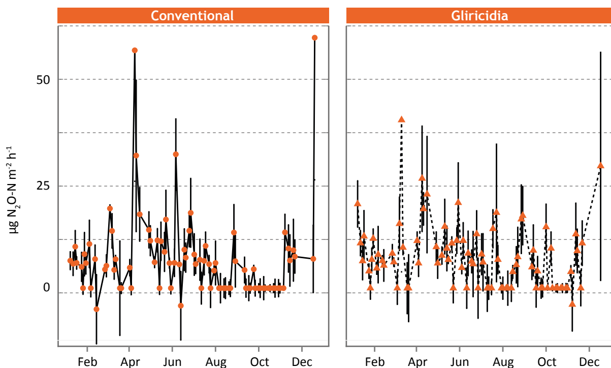
Figure 7. \text{N}_2\text{O} fluxes from the conventional and Gliricidia treatments measured over 84 sampling points in 2013. Vertical bars are standard error across six chambers. Fluxes below detection limit were set to zero in accordance with good practice (Parkin et al. , 2012) but graphed, with standard error, to show variability. The variation within and between treatments can complicate the production of robust GHG estimates. Sampling methodology should be considered when evaluating the robustness of GHG emissions and C sequestration data.
