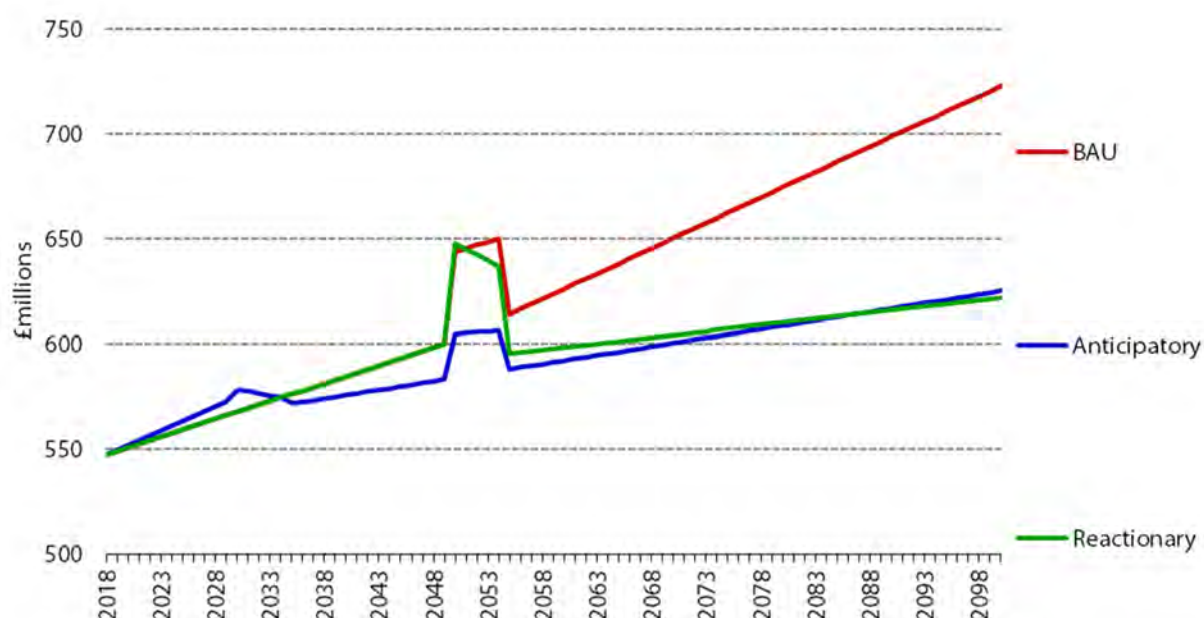
Figure 3.7. Norfolk and Suffolk broads case study: Long-term pattern of costs (£m) under different adaptation scenarios
