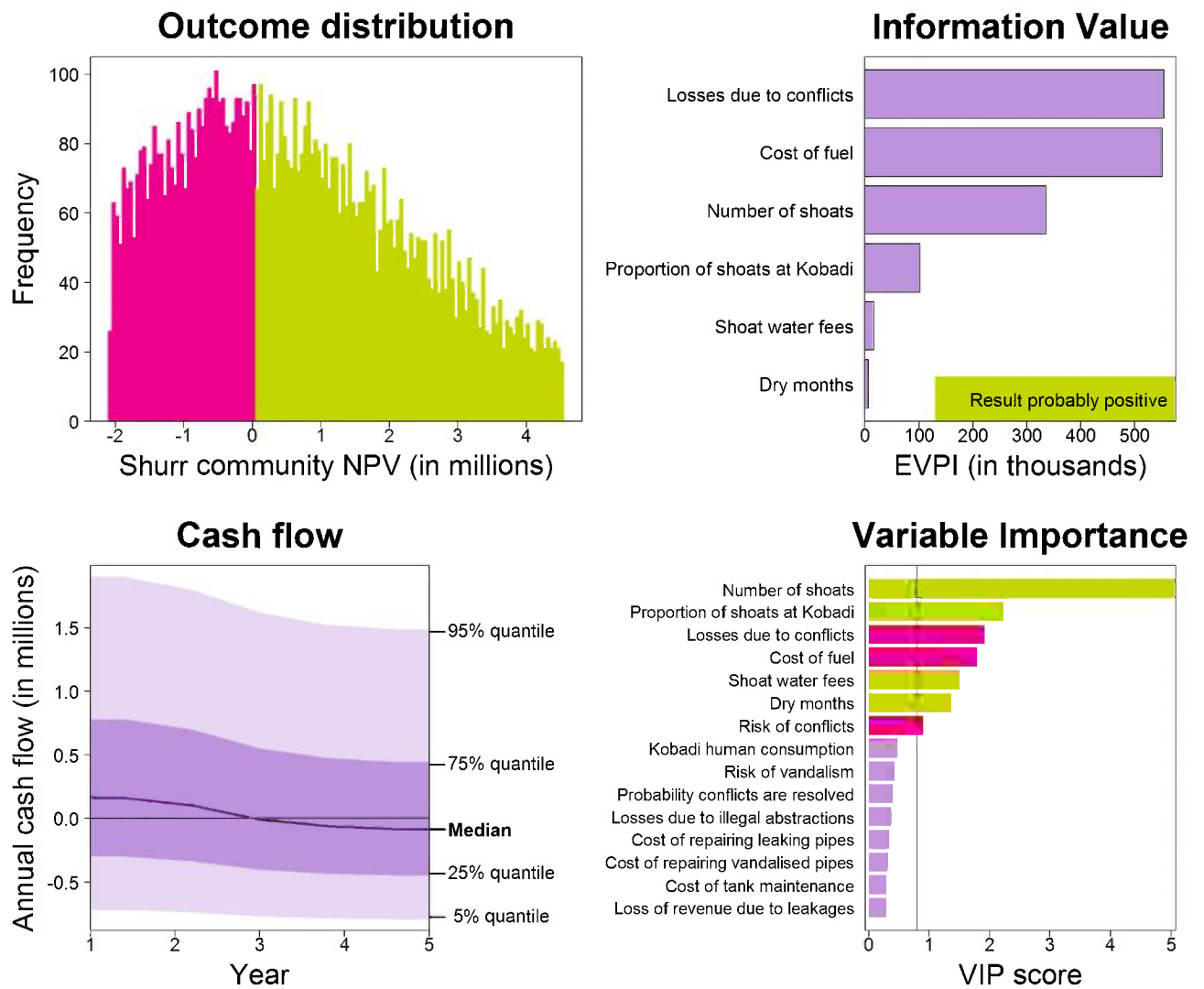
Figure 11: Simulation results: Community NPV of constructing an above-ground concrete water tank with a steel water piping system
