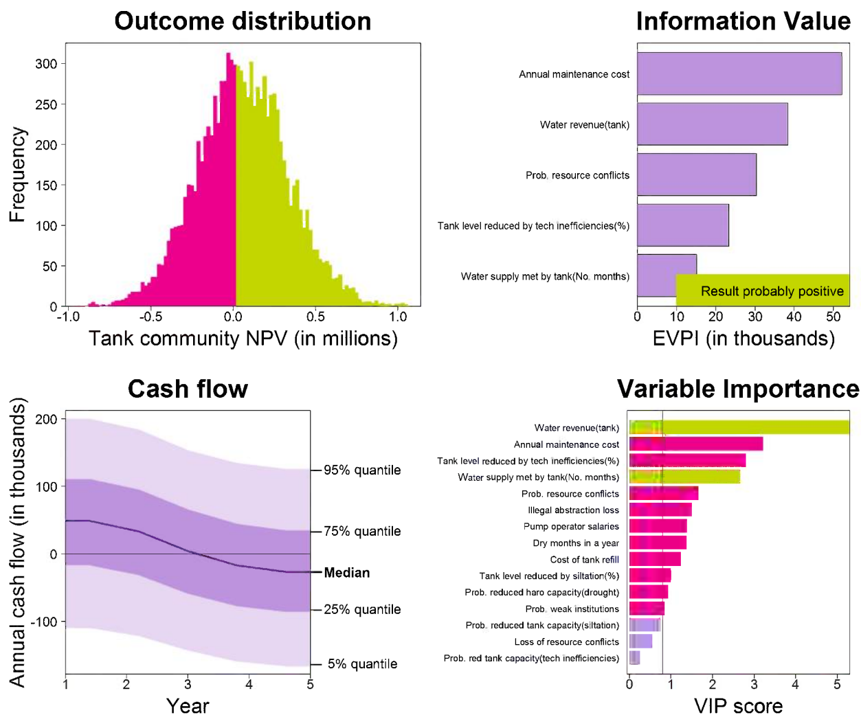
Figure 8: Simulation results: Community NPV of constructing the underground water tank
