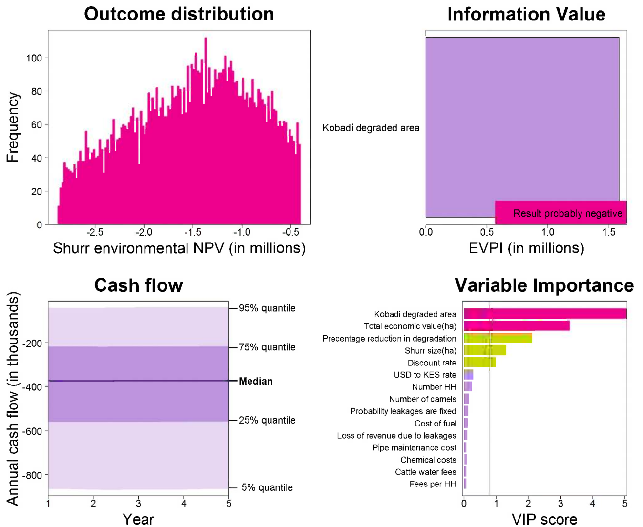
Figure 12: Simulation results Environmental NPV of constructing an above-ground concrete water tank with a steel water piping system
