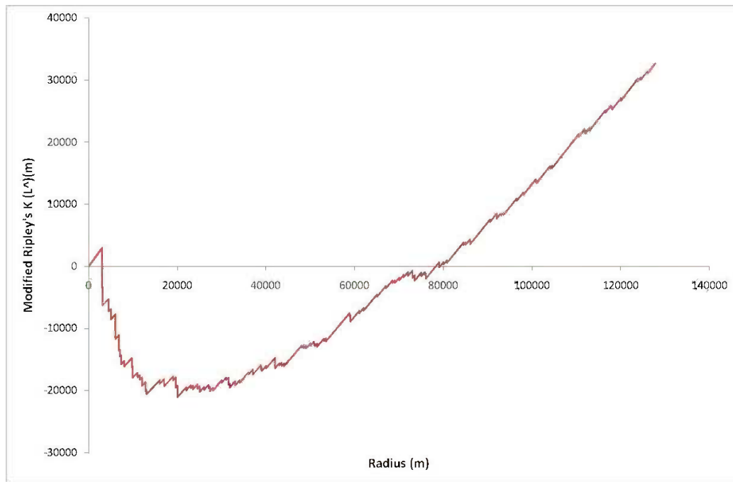
Figure 12 Results of Ripley's K analysis on one-dimensional data of barriers along the lower and middle Orange River. Values of zero reflect random distributions, while values < 0 indicate clumping and values > 0 indicate regular spacing.
