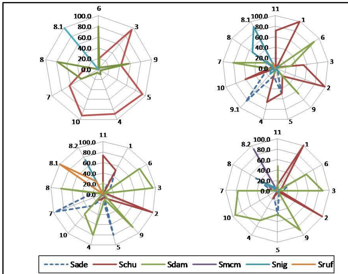
Figure 30 Radar diagrams showing percentage contributions of six blackfly species at each site over four sampling visits. Clockwise from top left: November 2015; March 2016; July 2016; December 2016
