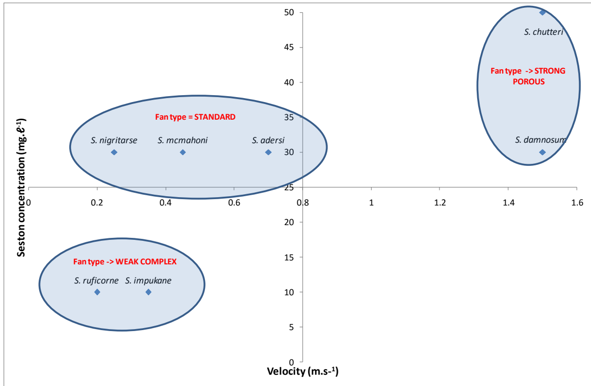
Figure 9 Conceptual grouping of Orange River blackfly species, based on seston concentration and velocity preferences (Palmer and Craig 2000)
