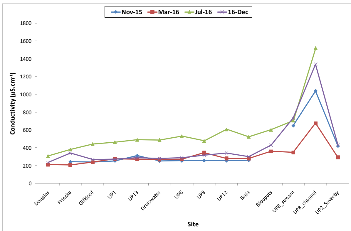
Figure 21 Conductivity values for late spring (November 2015), late summer (March 2016), winter (July 2016) and early summer (December 2016) for study sites, going from upstream to downstream
