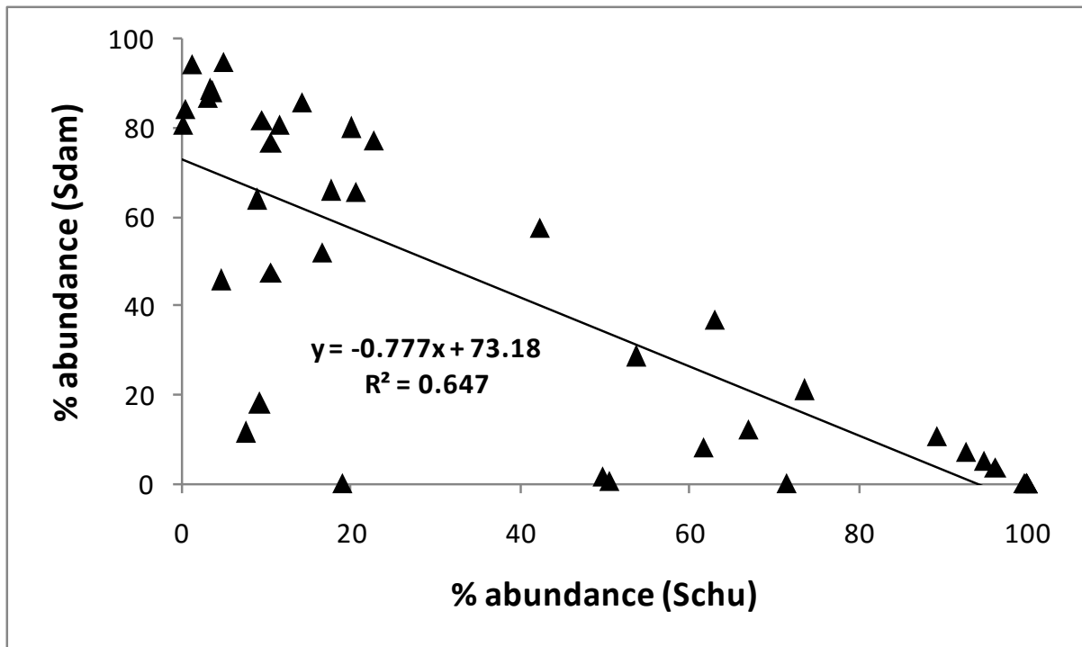
Figure 32 Negative correlation between abundances of Simulium. chatteri and S. damnosum
