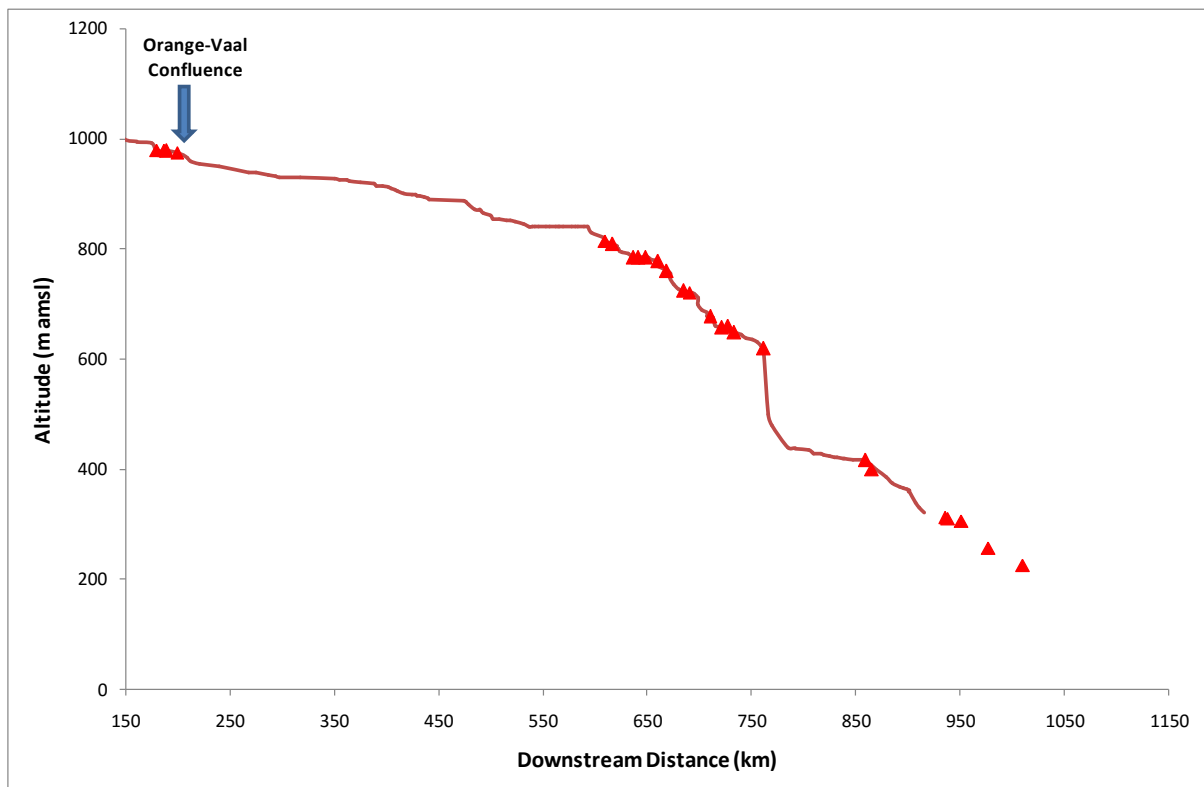
Figure 11 Distribution of multiple-channelled sites on the Orange River downstream of van der Kloof Dam
