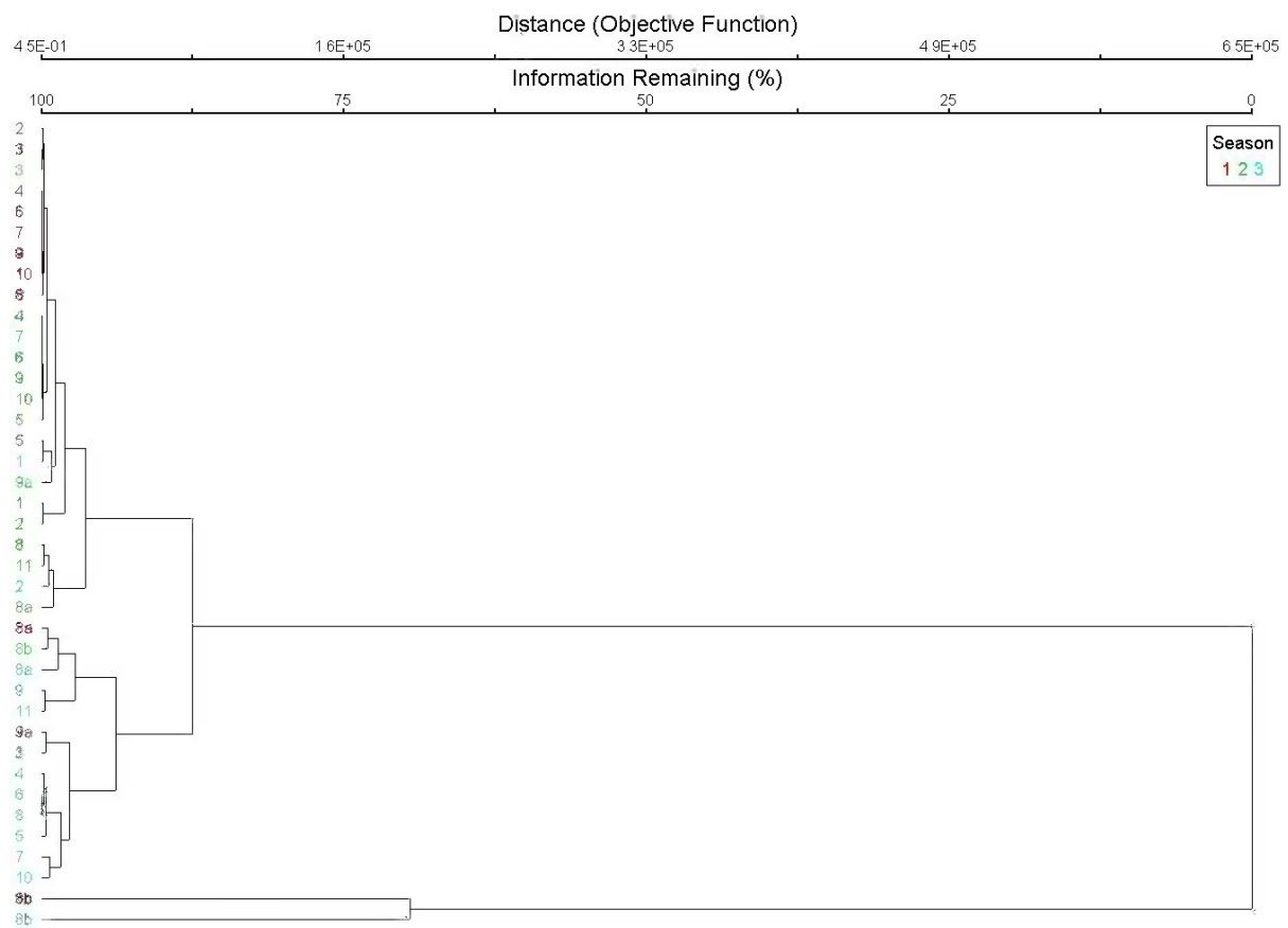
Figure 43 Cluster analysis of study sites based on water quality variables
