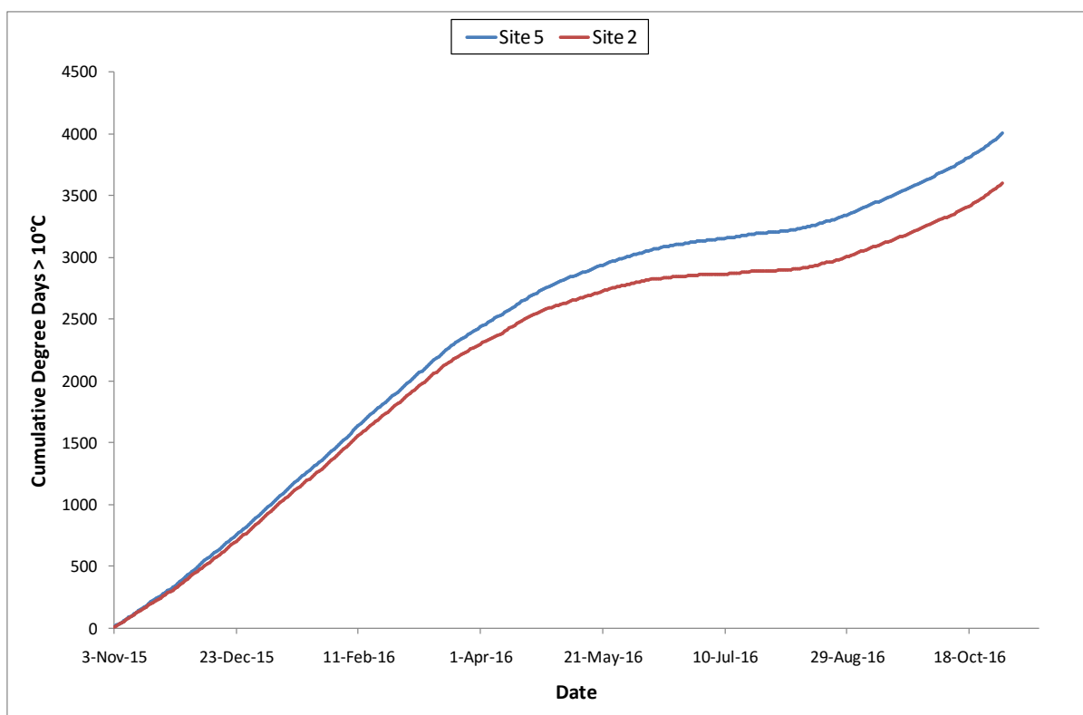
Figure 25 Cumulative degree days > 10°C for sites 2 (Prieska) and 5 (Sun River Lodge, Upington) based on mean daily water temperatures from 3 November 2015 – 2 November 2016
