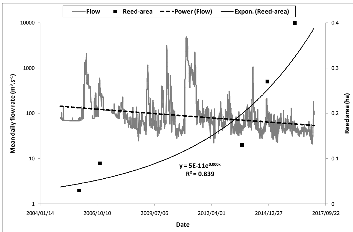
Figure 40 Change in reed area over a thirteen-year period at site 2, and corresponding mean daily flow rate time series for gauging weir D7H002 (Prieska)
