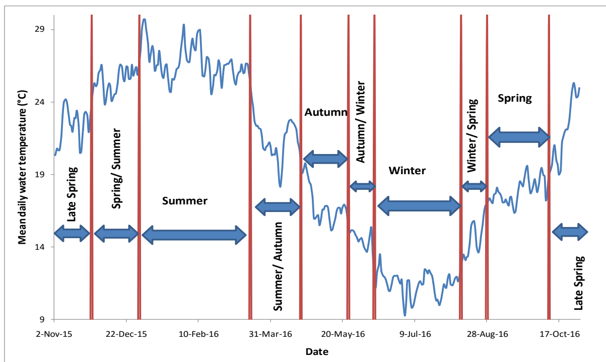
Figure 28 Significant thermal regime shifts for mean daily water temperatures at Prieska, whereby the annual thermograph has been divided into distinct thermal seasons
