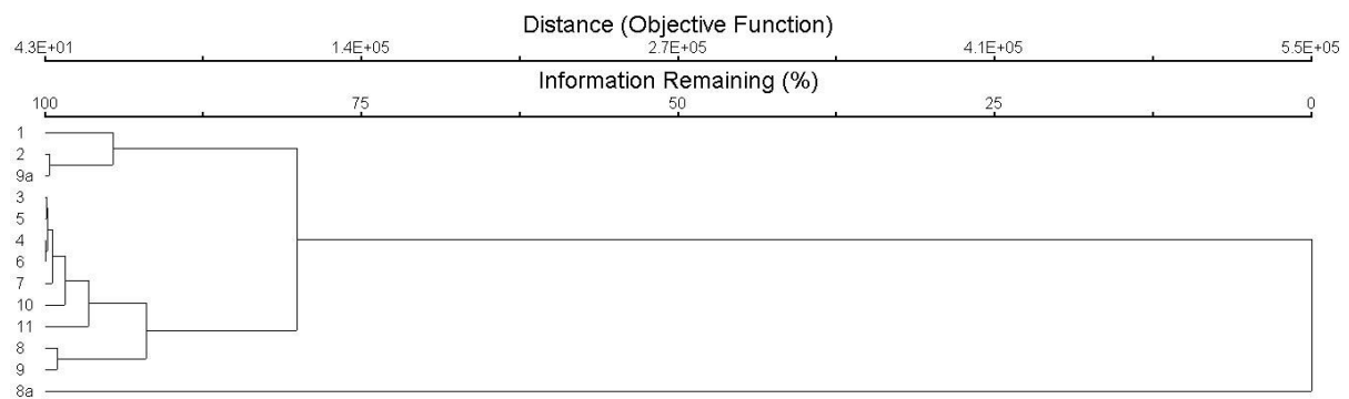
Figure 45 Cluster classification of study sites based on water temperature metrics
