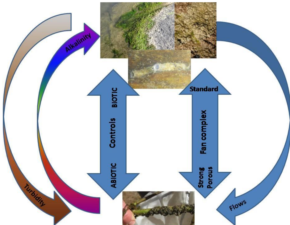
Figure 50 Conceptual model of abiotic-biotic interactions as they relate to switching of dominant species states
