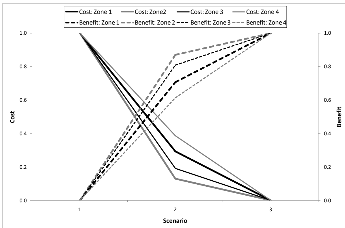
Figure 46 Cost-benefit curves standardised to scores between 0 and 1, for three management scenarios (1 = base; 2 = optimistic; 3 = pessimistic) and four economic zones
