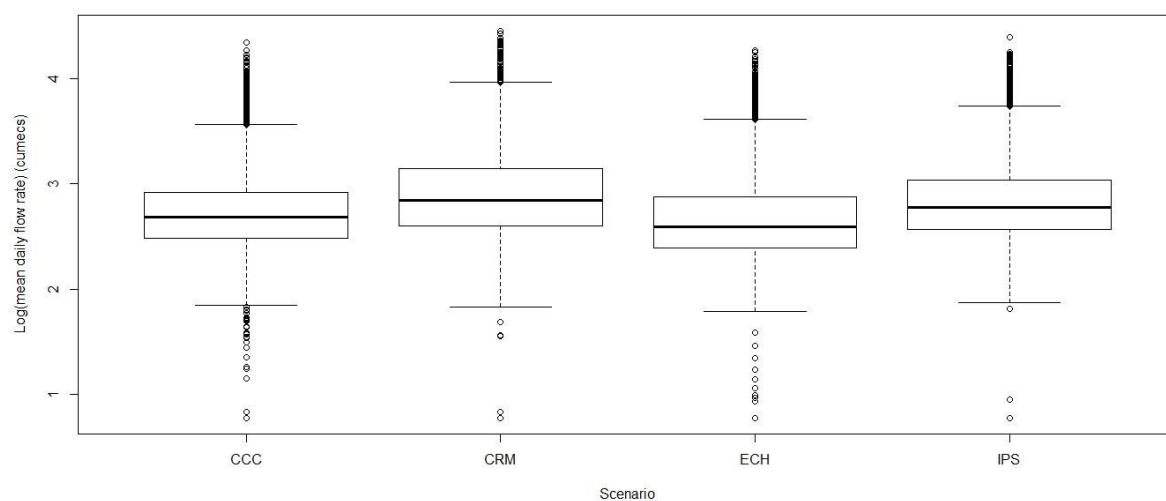
Figure 15 Box-and-Whisker plot of flows for four intermediate future climate change models for quinary 2025, corresponding with D7H005 at Upington
