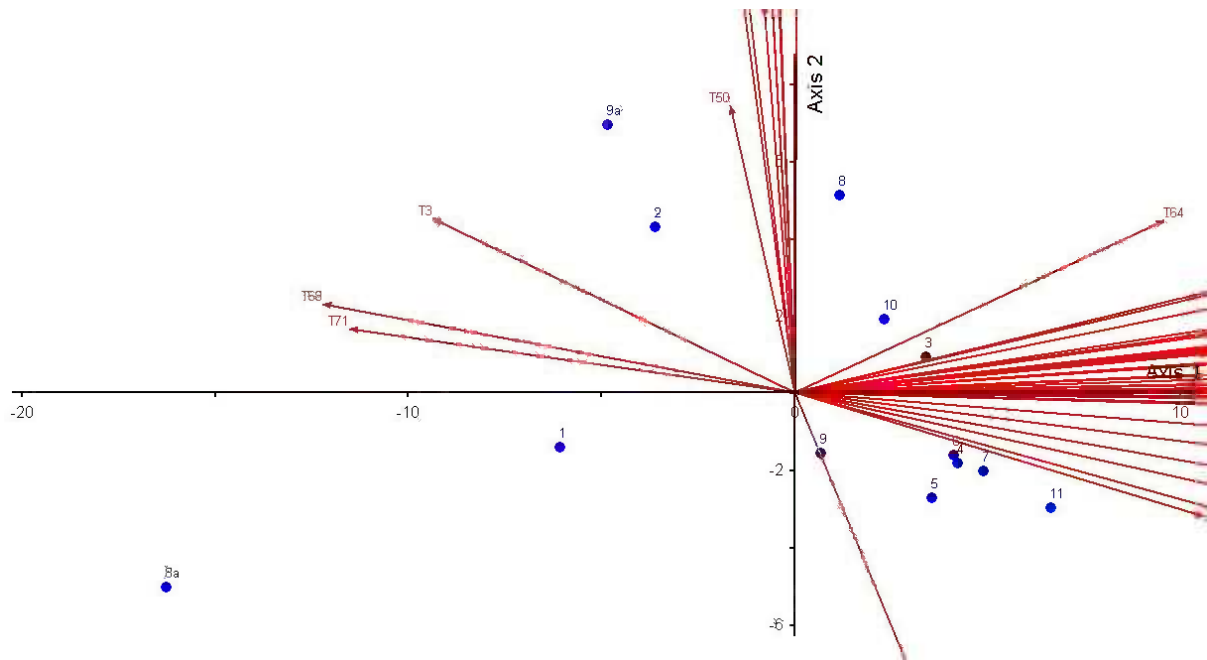
Figure 44 Principal Components Analysis of study sites based on water temperature metrics. PC axes 1-2 contributed to 65.6 and 86.9% of site variation.
