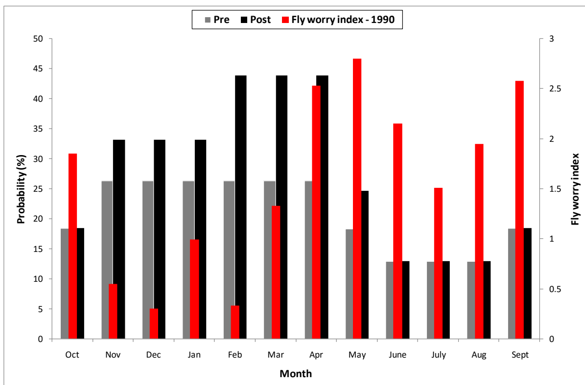
Figure 49 Seasonal variation in blackfly outbreak probabilities for pre- and post-impoundment flow conditions
