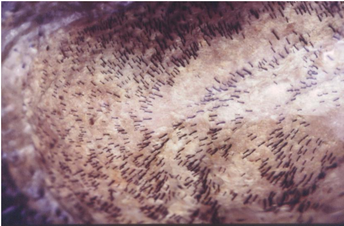
Figure 4 Example of blackfly larvae in situ on rocky substrate, with larval densities scoring a 7 using Palmer's (1994) scoring system.
