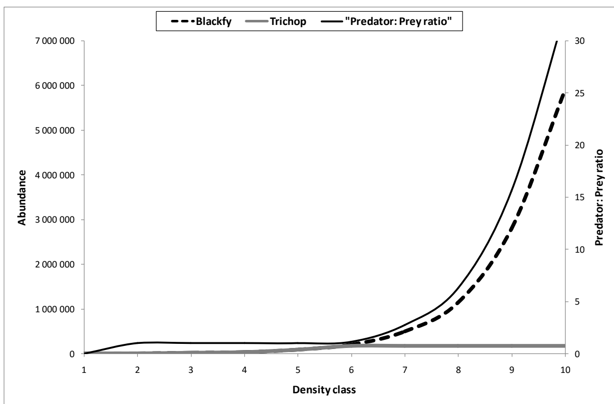
Figure 39 Potential numbers of blackfly and caseless caddisfly larvae as a function of density classes for a habitat area of 90 000 cm 2 , and associated predator: prey ratios
