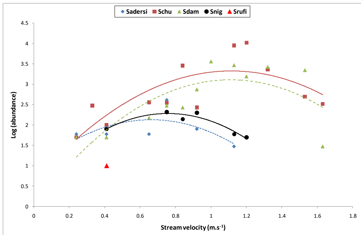
Figure 34 Log-transformed abundances of five species of blackfly based on combined sample data from November 2015 and March 2016. Velocity preference curves are based on maximum abundances for velocity values (see Table 8).
