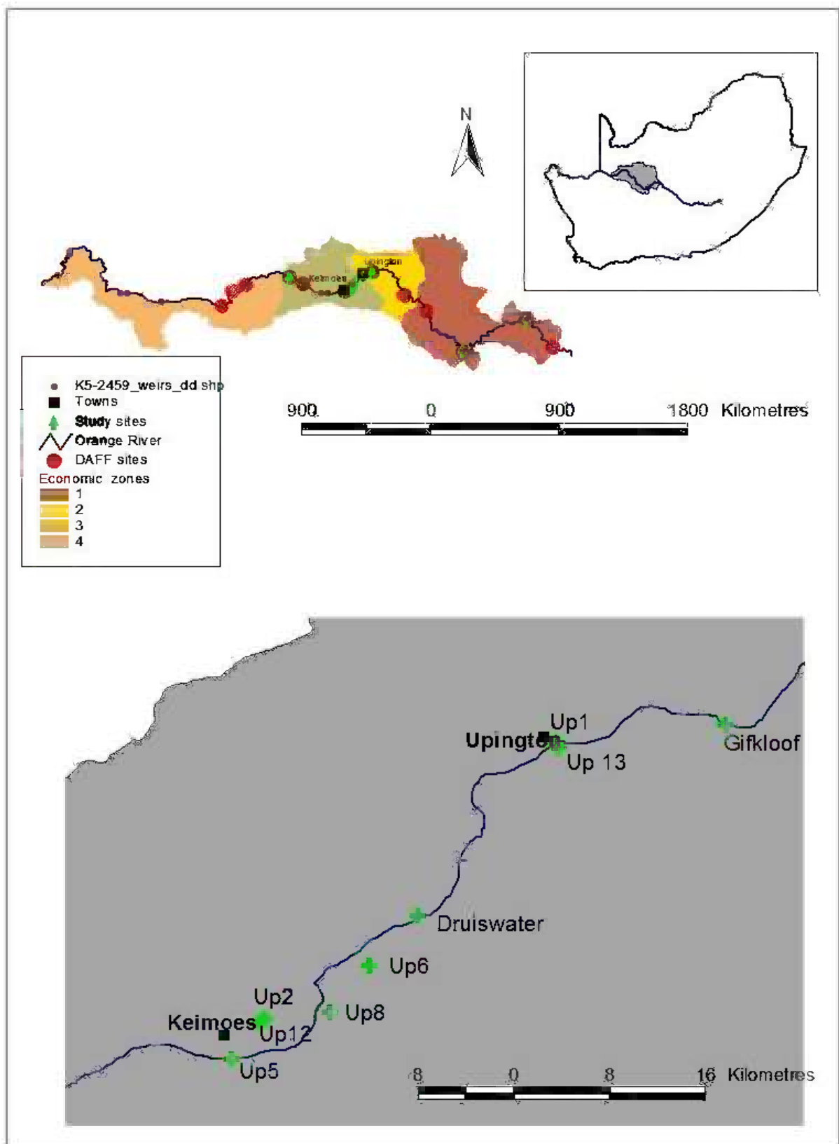
Figure 6 Map of study area within context of economic zones used by Mullins (2007) (top) and within context of South Africa (inset). Clustering of sites between Upington are shown in more detailed the lower figure
