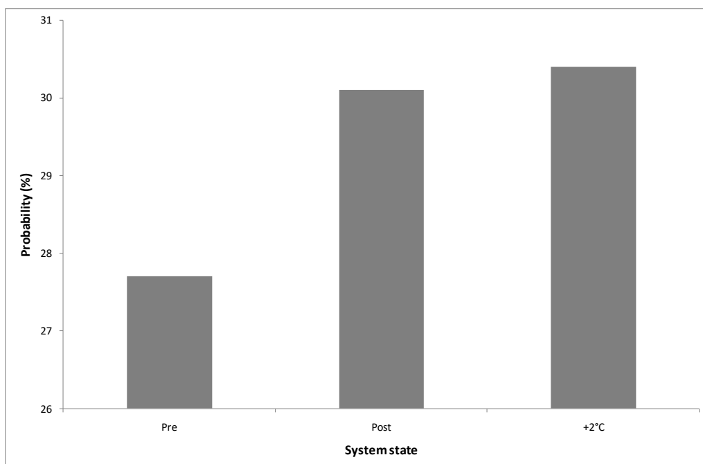
Figure 48 Probability of blackfly outbreaks under pre-impoundment, post-impoundment and future global climate change scenarios
