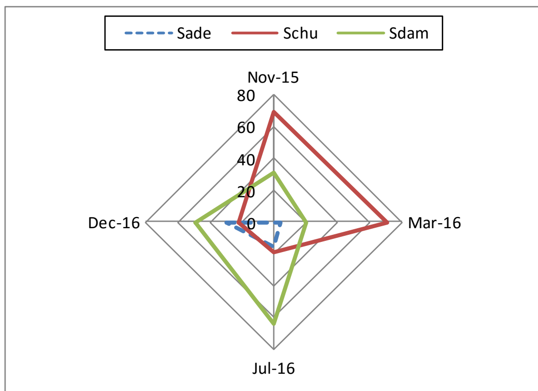
Figure 29 Radar diagram showing the percentage contribution of the three most dominant species of blackfly sampled across all sites and seasons
