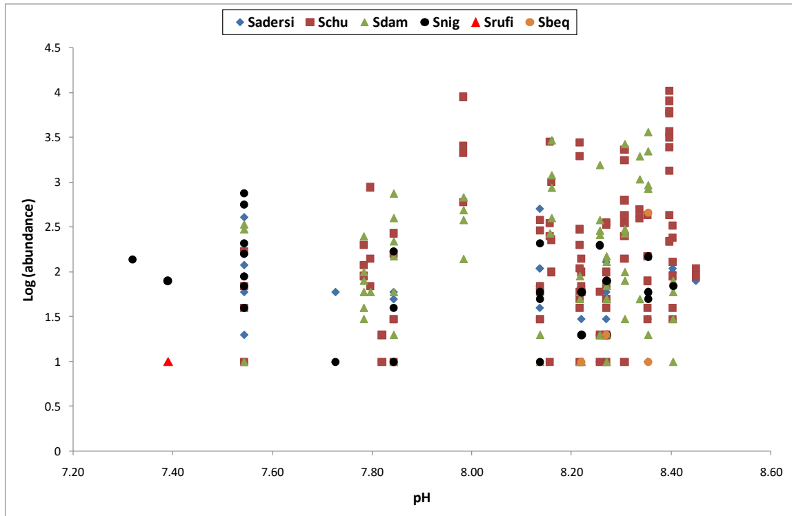
Figure 37 Scatterplot of log-transformed abundances of six species of blackfly based on combined sample data from November 2015 and March 2016 versus pH values.
