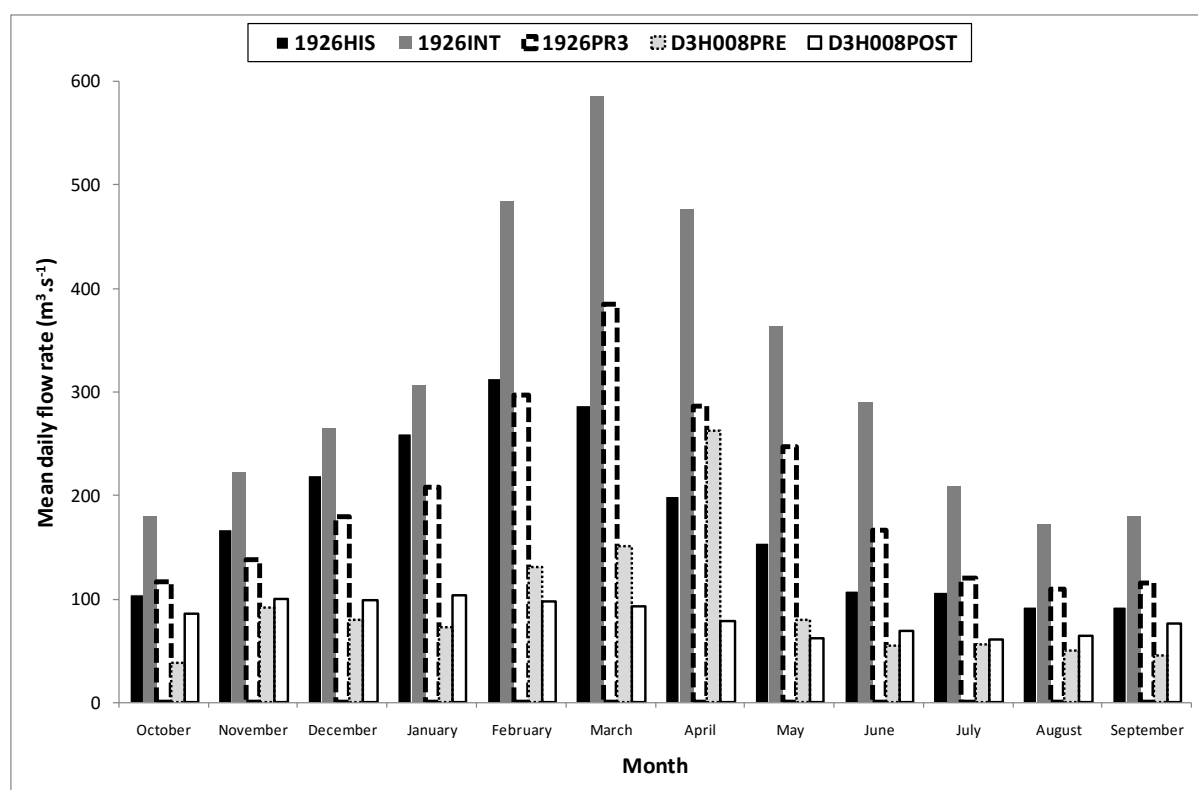
Figure 16 Median daily flow rates per month for five flow time series
