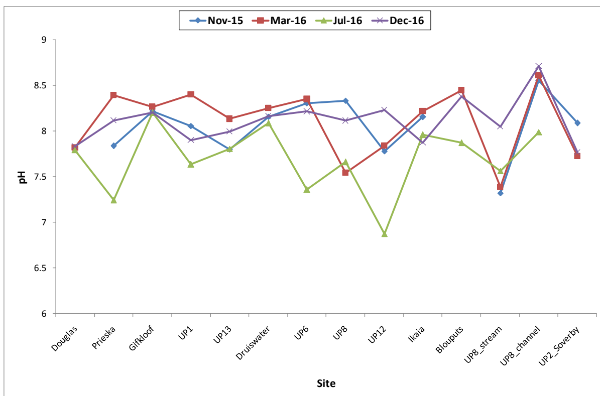
Figure 20 pH values for late spring (November 2015), early summer (March 2016), winter (July 2016) and early summer (December 2016) for study sites, going from upstream to downstream
