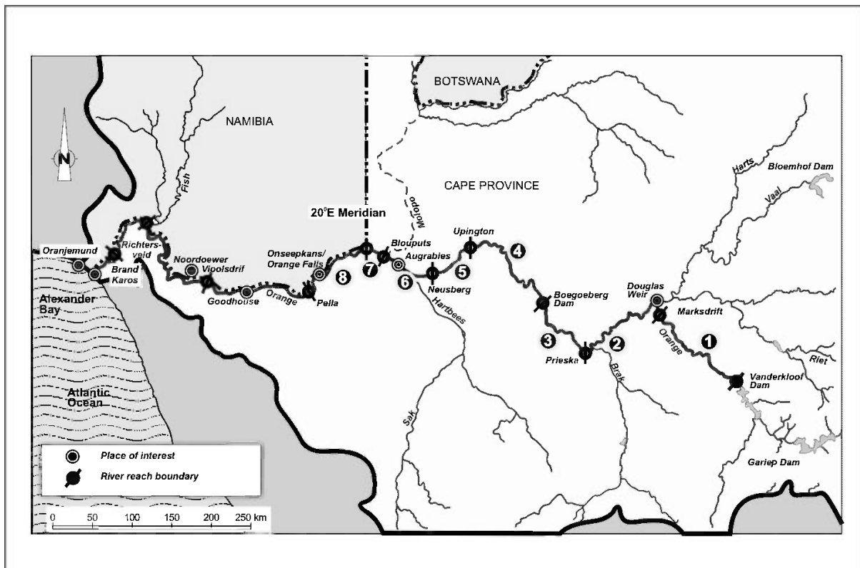
Figure 1 General locality map of the middle and lower Orange River, and reflecting extent of main pest blackfly control programme. Numbers reflect river reach zones used by Palmer et al. (2007) for hydrological modelling.
