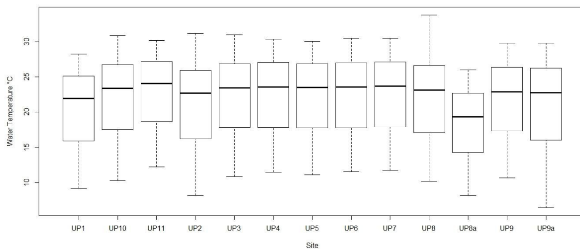
Figure 24 Box-and-whisker plots of water temperatures for 13 study sites, showing median values and 25 th / 75 th percentiles, and minima and maxima per site reflected as “whiskers”
