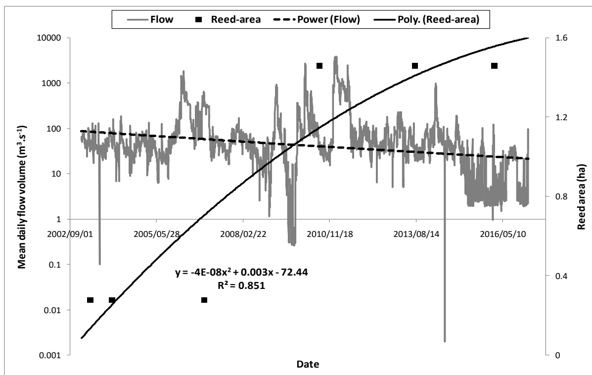
Figure 41 Change in reed area over a thirteen-year period at site 11, and corresponding mean daily flow rate time series for gauging weir D7H014 (Neusberg)
