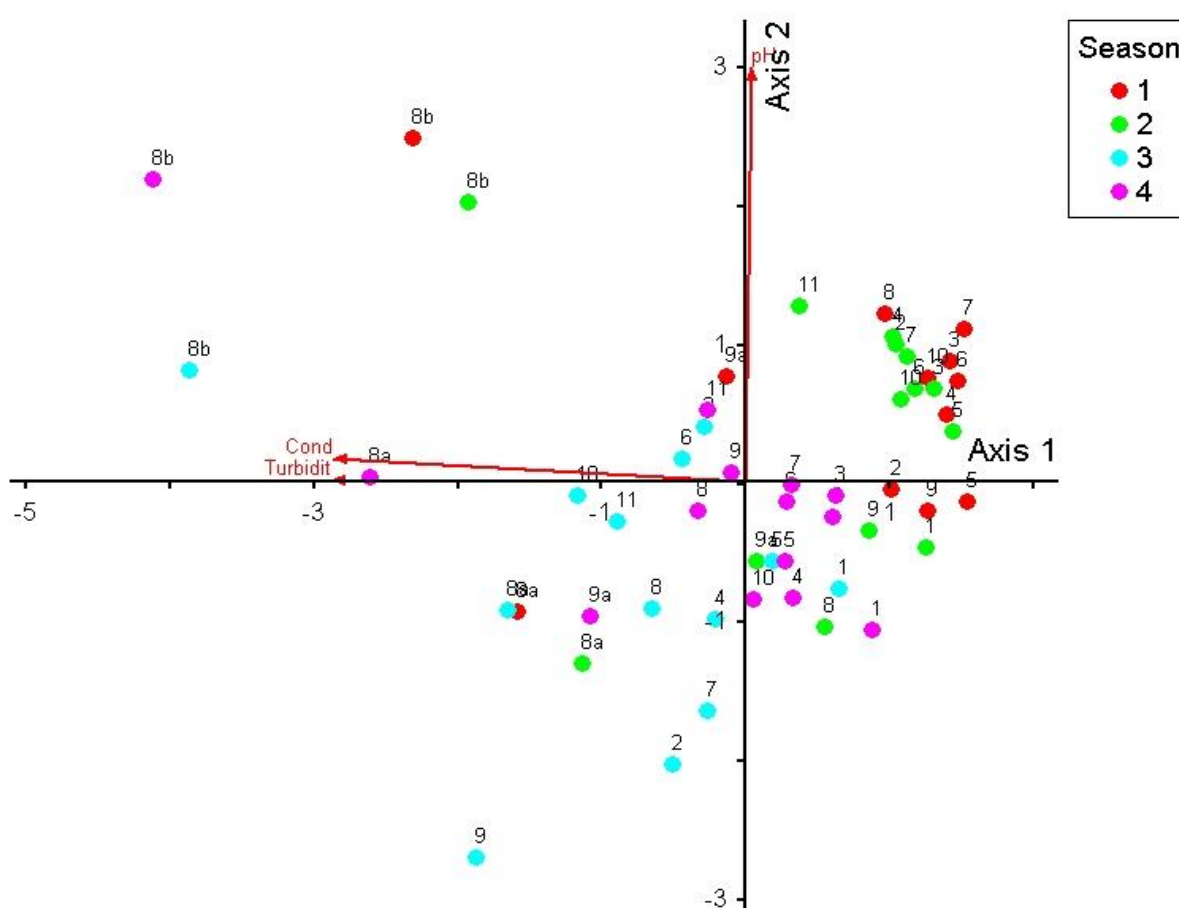
Figure 42 Principal Components Analysis of study sites based on water quality variables for November 2015, March, July and December 2016. Seasons 1-4 represent the data collected for the late spring (November 2015), late summer (March 2016), winter (July 2016) and early summer (December 2016) sampling periods respectively.
