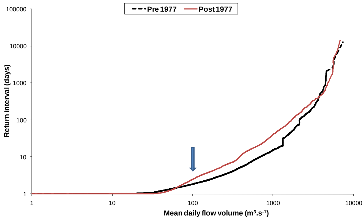
Figure 13 Return interval curves for gauging weir Up7H005 (Uppington) for pre- and post-impoundment periods (1942-1977 and 1978-2016)
