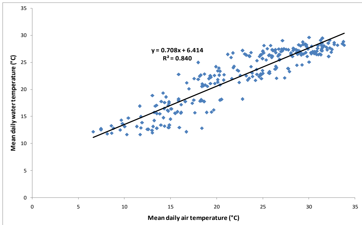
Figure 27 Linear regression between mean daily water temperatures for study site 5 and air temperature logger located at DAFF office, Upington
