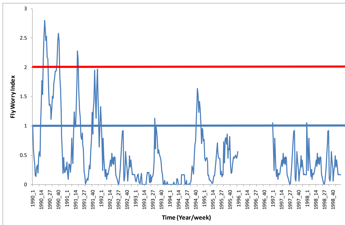
Figure 10 Fly Worry Index scores on a weekly basis from 1990-1998, where date suffixes represent weeks of the year. The scores from multiple users are averaged, and are based on discrete values, where 0 = no flies; 1 = some flies; 2 = moderate levels of annoyance, and 3 = extreme levels of annoyance (Palmer, 2017, unpub. data)
