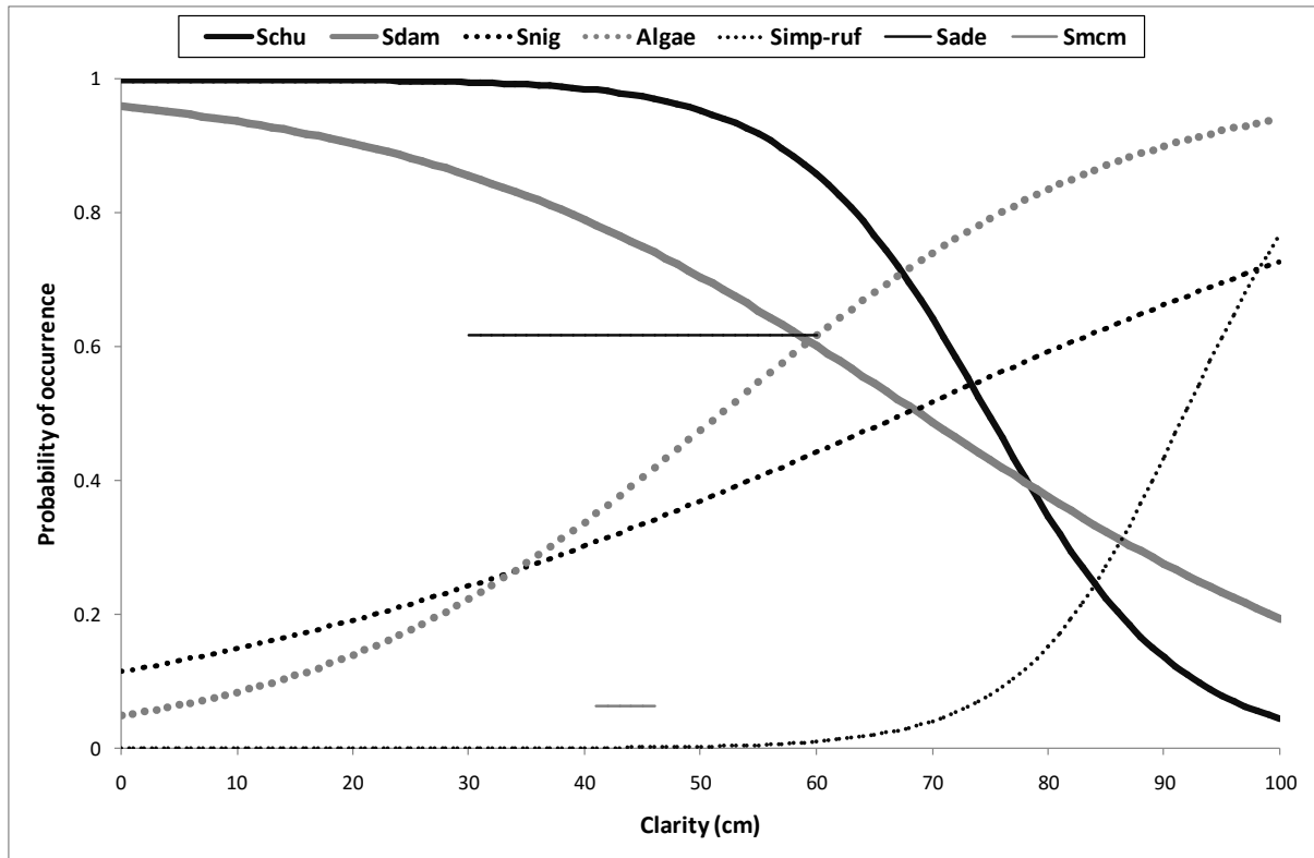
Figure 36 Probability of occurrence of seven blackfly species as a function of water clarity (cm), and benthic algae
