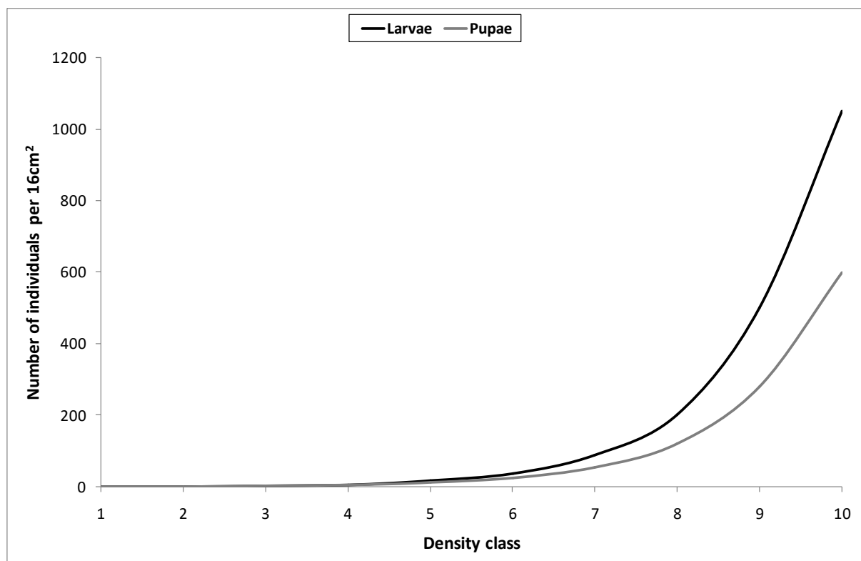
Figure A1 Logarithmic relationship between numbers of blackfly larvae and pupae versus the ten-point scores from Palmer (1994)
