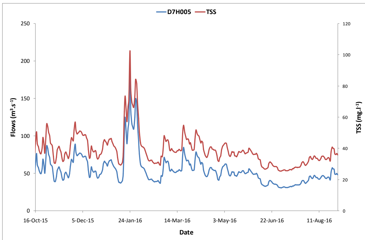
Figure 18 Plot of mean daily flow volumes and seston concentration
