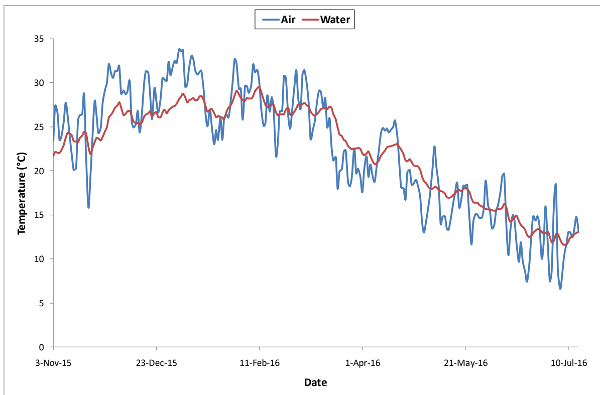
Figure 23 Hourly water and air temperature data for site 5 (Sun River Lodge, Upington) from 4 November 2015 – 10 July 2016
