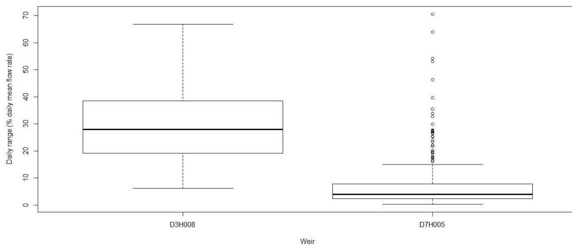
Figure 14 Box-and-Whisker plot of 12-minute interval subdaily flow range as a percentage of daily mean flow rate for site 1 (Douglas – D3H008) and site 4 (Uppington – D7H0005) for 1 October 2015 – 30 September 2016
