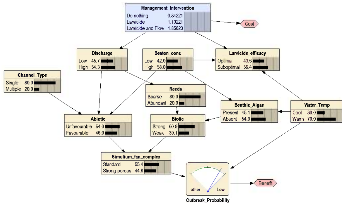
Figure 47 Bayesian network model, showing parent and child nodes together with management and utility nodes
