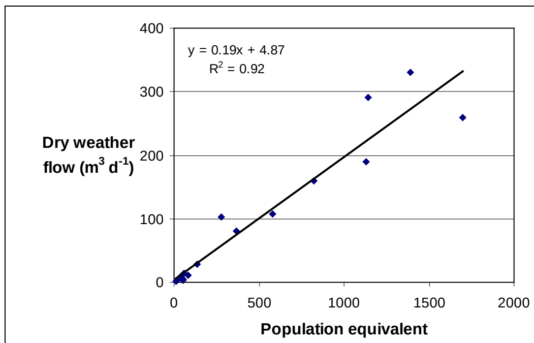
Figure 6.14 Relationship between dry weather flow consents and population equivalent values for small sewage works (PE = \leq 2000 ) in Bure and Ant subcatchments of the Broads.
