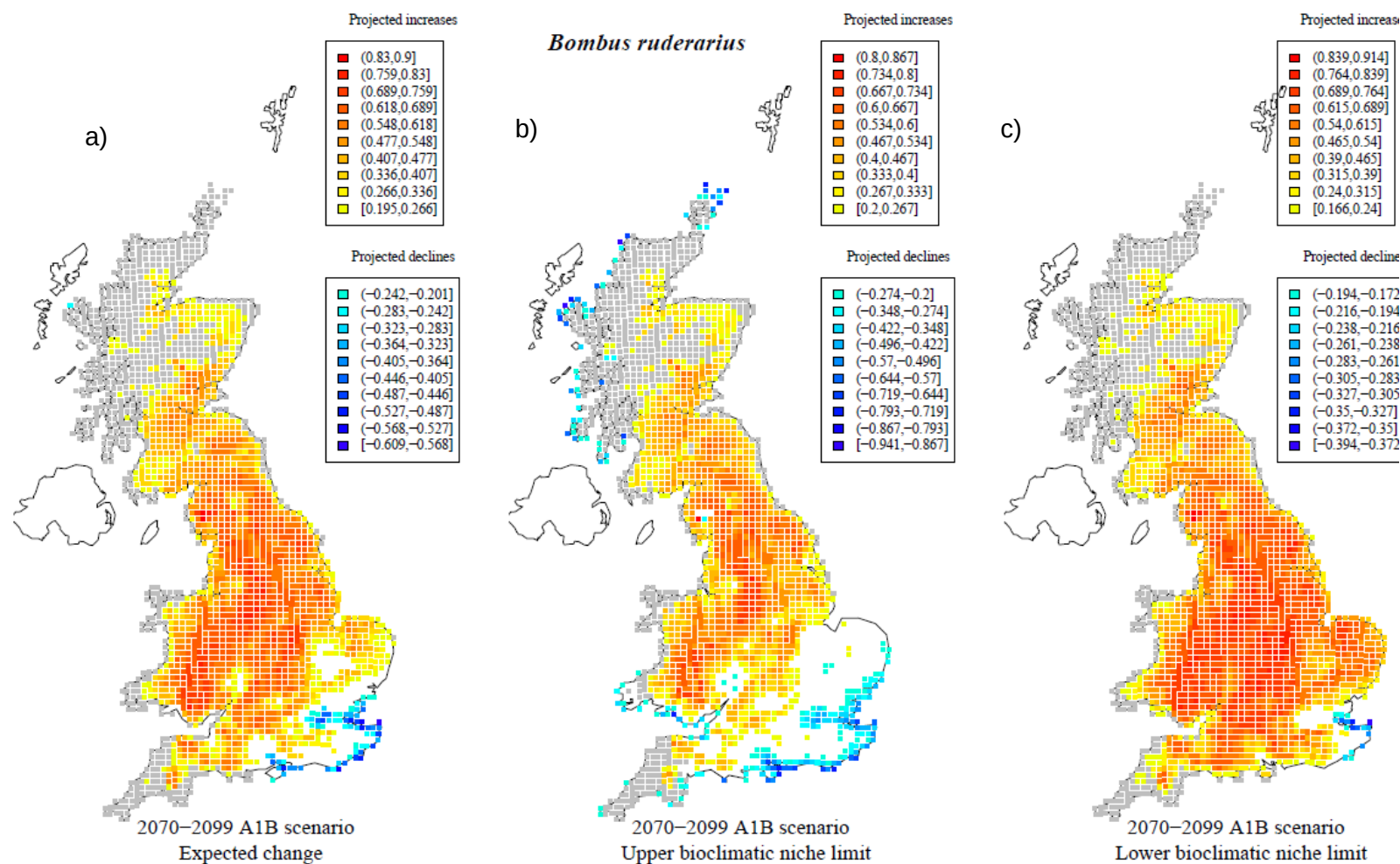
Figure 4.2 Maps showing a) Projected change in modelled probability of suitable climate space for Bombus ruderarius coloured to delineate different climate zones (the same as Figure 1c); b) and c) Projected future change in probability of suitable climate space for Bombus ruderarius in relation to the upper and lower 95% confidence intervals for the modelled historic probability of occurrence. Colours as in Figure 4.1
