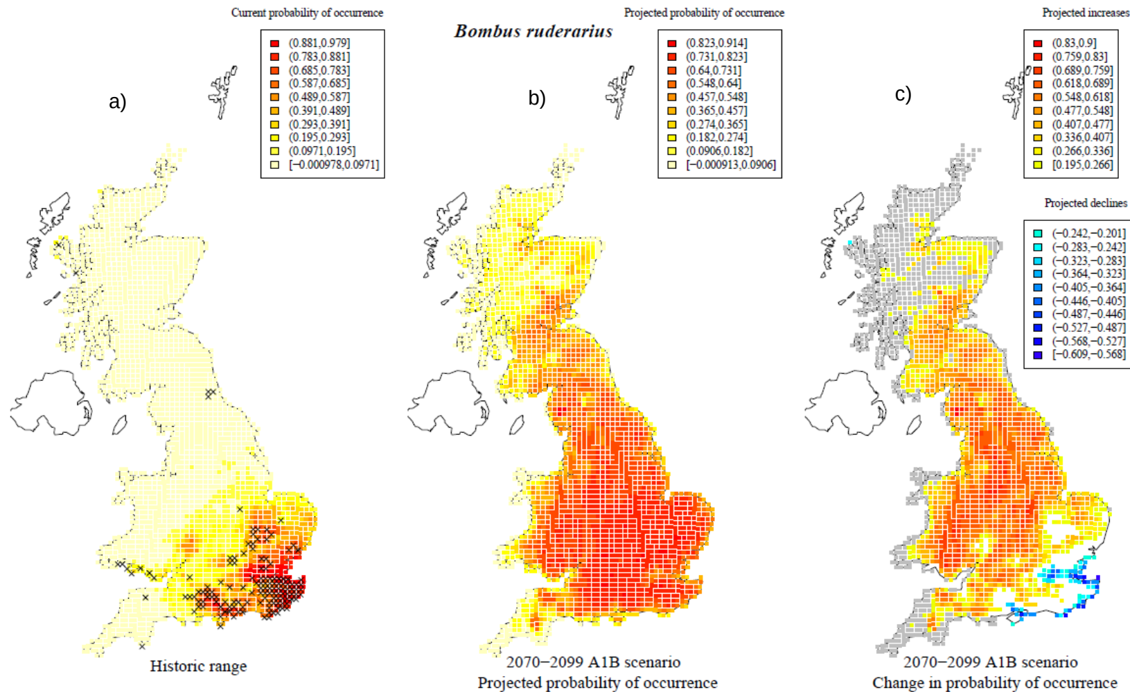
Figure 4.1 Maps showing a) historic distribution of an example species, Bombus ruderrarius . Black crosses show submitted records, coloured squares show modelled probability of historic (1970-1990) occurrence; b) Projected probability of occurrence under A1B scenario; c) The change in modelled probability of occurrence coloured to delineate different climate zones (see main text) - yellow and red squares show areas of new climate space, white squares show areas of climate overlap, blue squares show adversely sensitive areas and grey squares indicate areas climatically unsuitable in both periods
