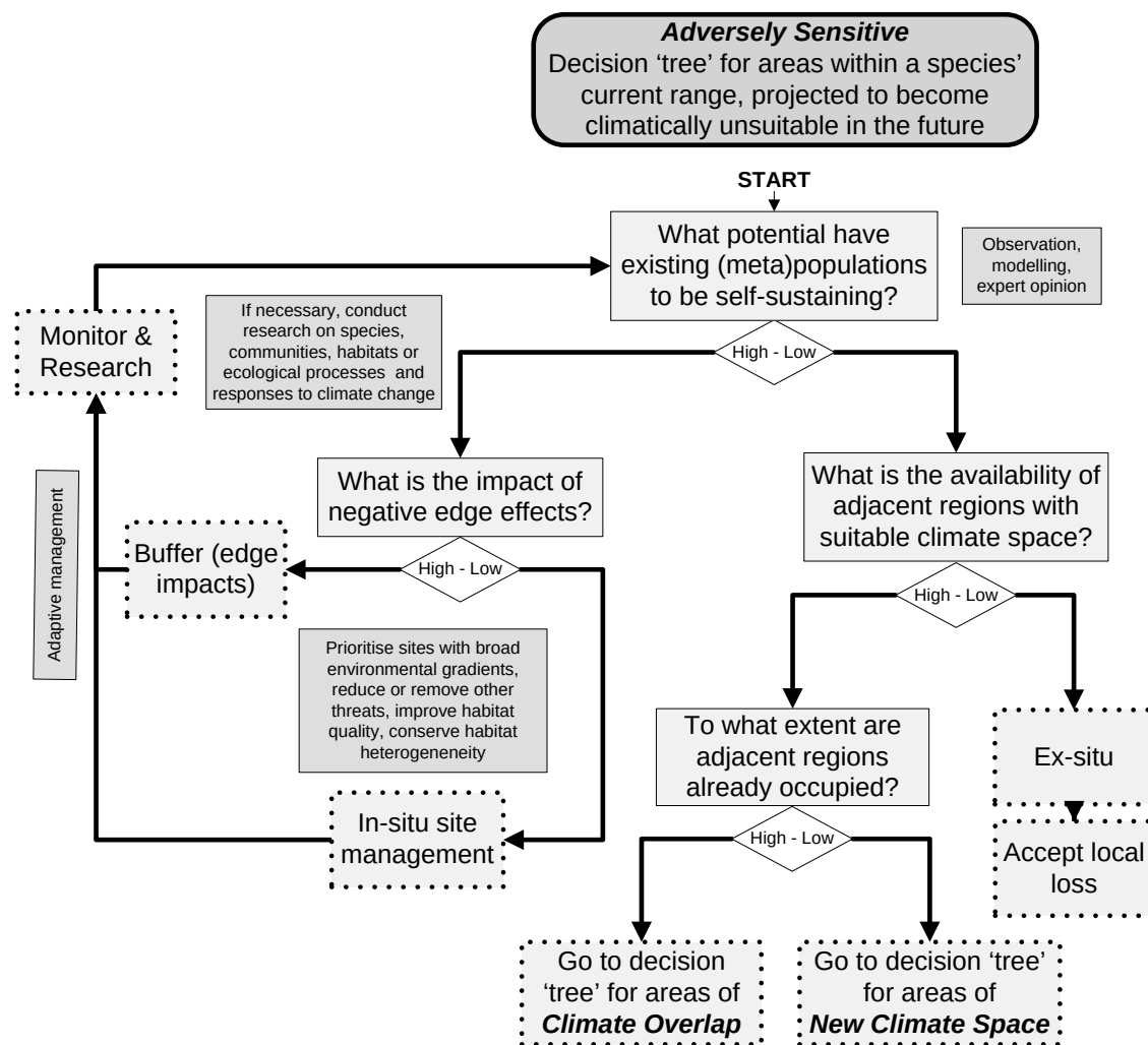
Figure 4.5 Decision tree for Adversely Sensitive Areas (reproduced from Oliver et al. 2012). Light grey boxes with solid borders indicate questions whose answers lead to different routes through the tree. If the answer to a question is uncertain, then multiple routes should be taken through the tree simultaneously. Light grey boxes with dashed borders indicate suggested adaptation actions, with relevant additional information in dark grey boxes
