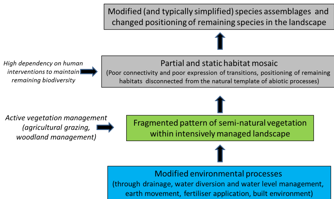
Figure 2.4 Functioning of modified landscape
