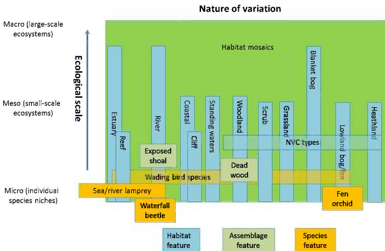
Figure 2.2 Wider ecological hierarchies and relationships (this is not intended to be exhaustive – in particular, only illustrative examples of smaller scale habitat features and assemblage/species features have been included).
