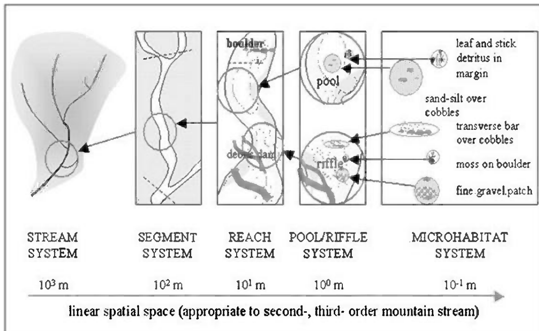
Figure 2.1 Example habitat hierarchy - river systems (after Frissell et al. 1986).
