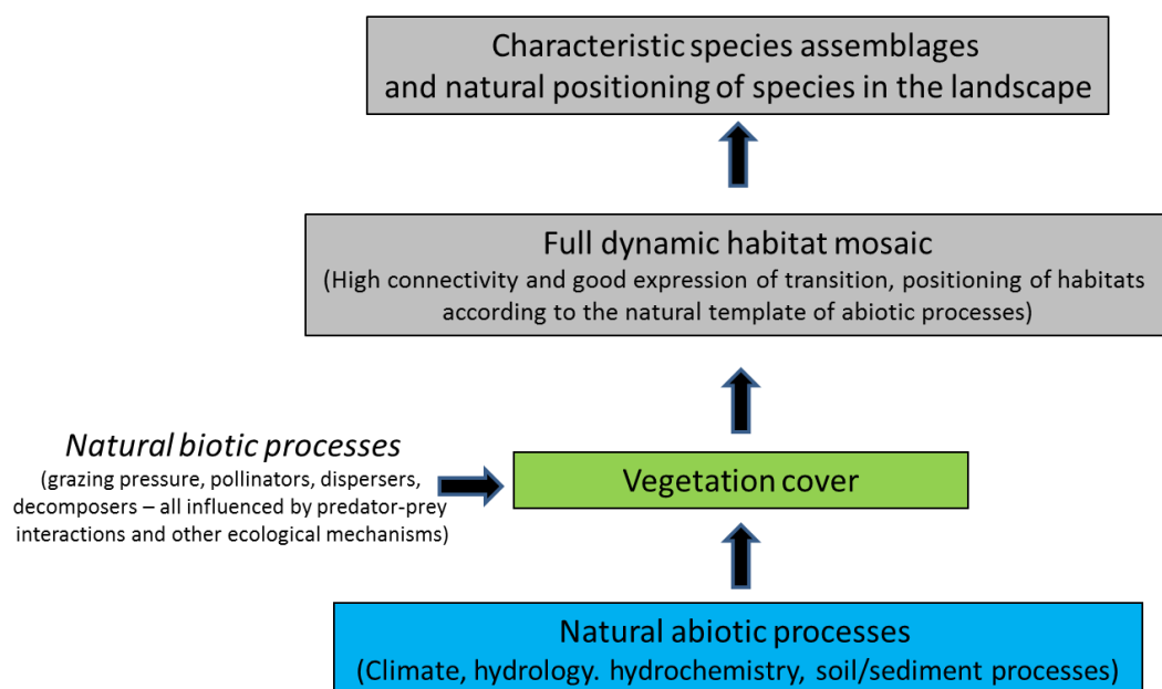
Figure 2.3. Naturally functioning landscape.
