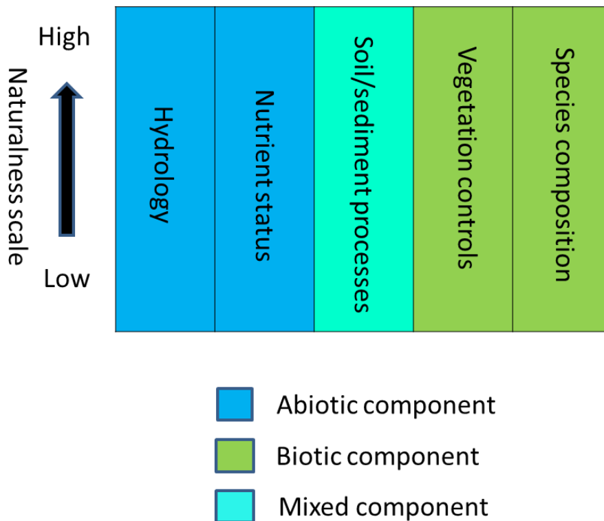
Figure 3.1 Natural process framework (applicable to a whole habitat resource or an individual site)
