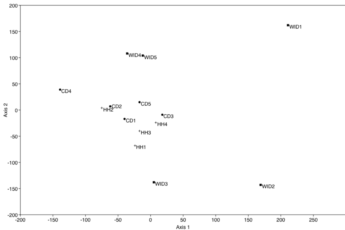
Figure 2 A) Non-metric multidimensional scaling (NMDS) and B) Detrended correspondence analysis (DCA) ordination plots of the fungal communities in the 14 quadrats in the Hardcastle Crag area.
