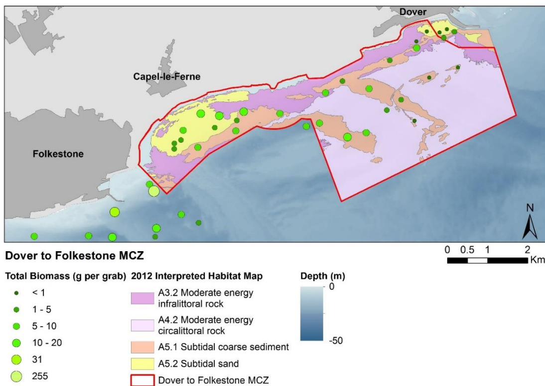
Figure 6. Spatial pattern of biomass (g wet weight) by Broadscale Habitat for Day Grabs sampled in the 2016 Dover to Folkestone MCZ survey (© Natural England and Environment Agency 2022).
