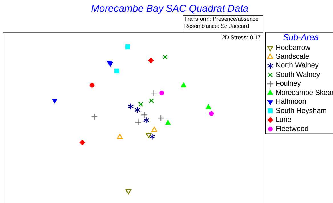
Figure 21 Morecambe Bay SAC Rocky Shore 2015 Non-metric Multidimensional Scaling (MDS) configuration plot of taxa presence/absence data using Jaccard similarity. Sample symbols are shown according to the area of Morecambe Bay in which the samples were taken. Sub-areas of the SAC are presented in the key from north (Hodbarrow on the Duddon Estuary) to south (Fleetwood on the southern coast at the mouth of Morecambe Bay).
