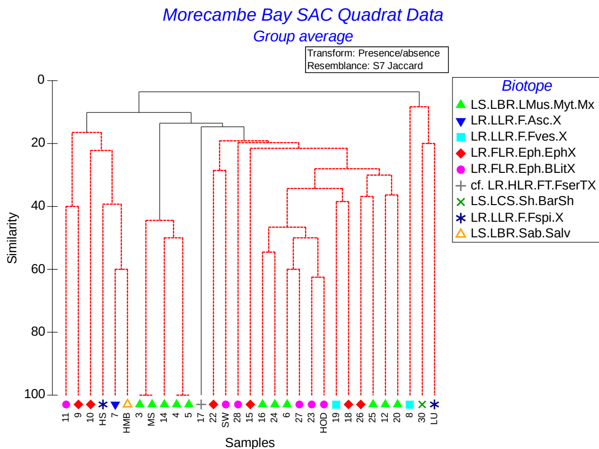
Figure 20 Morecambe Bay SAC Rocky Shore 2015 group average sorting dendrogram based on presence/absence transformed data. Samples presented by survey location with replicates combined for each site. Jaccard similarity and the SIMPROF test were used. Symbols are coded according to biotope.
