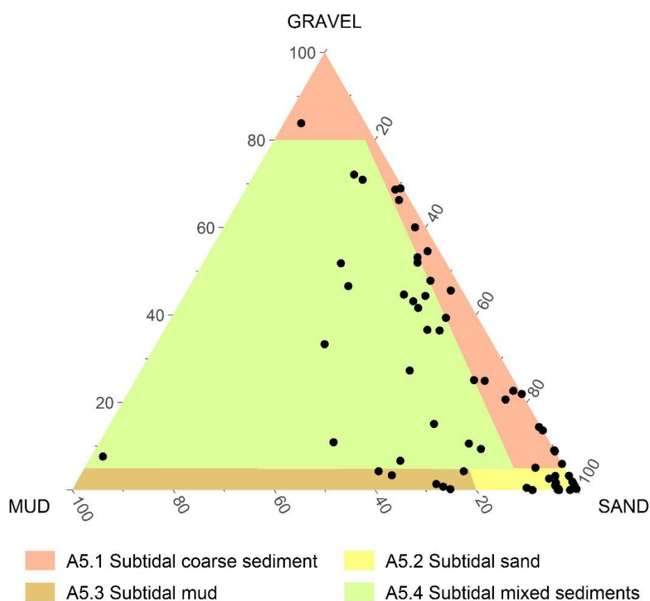
Figure 8. Classification of particle size distribution 0.5 phi ( \phi ) information for each 2017-18 Thanet Coast MCZ sample (closed black circles) into one of the sediment Broadscale Habitats (coloured areas) plotted on a true scale subdivision of the Folk triangle into the simplified classification for UKSeaMap (Long, 2006; Folk, 1954) (© Natural England and Environment Agency 2022).
