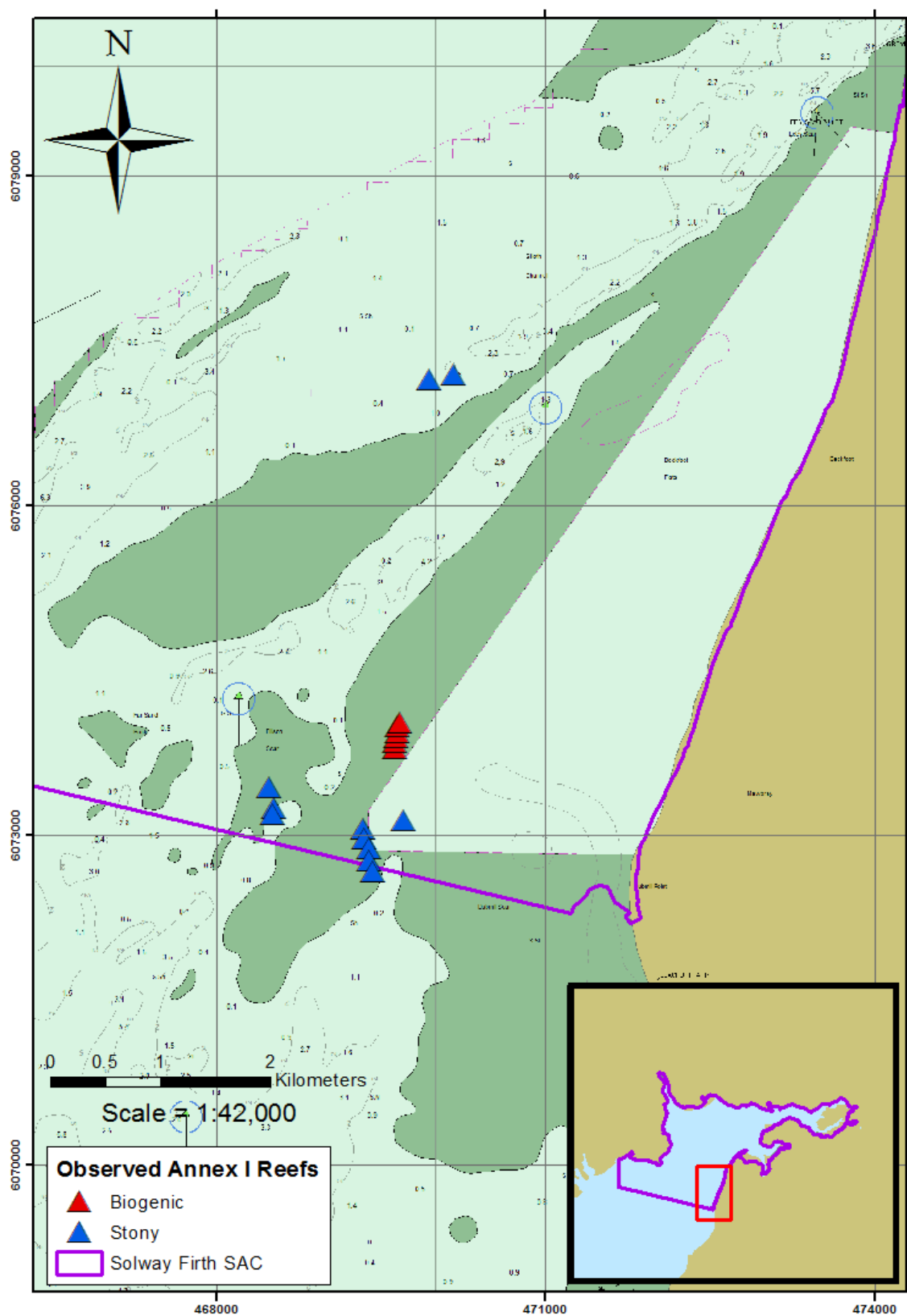
Figure 3.10: Distribution of observed potential Annex I reef features in the Solway Firth SAC survey area.
