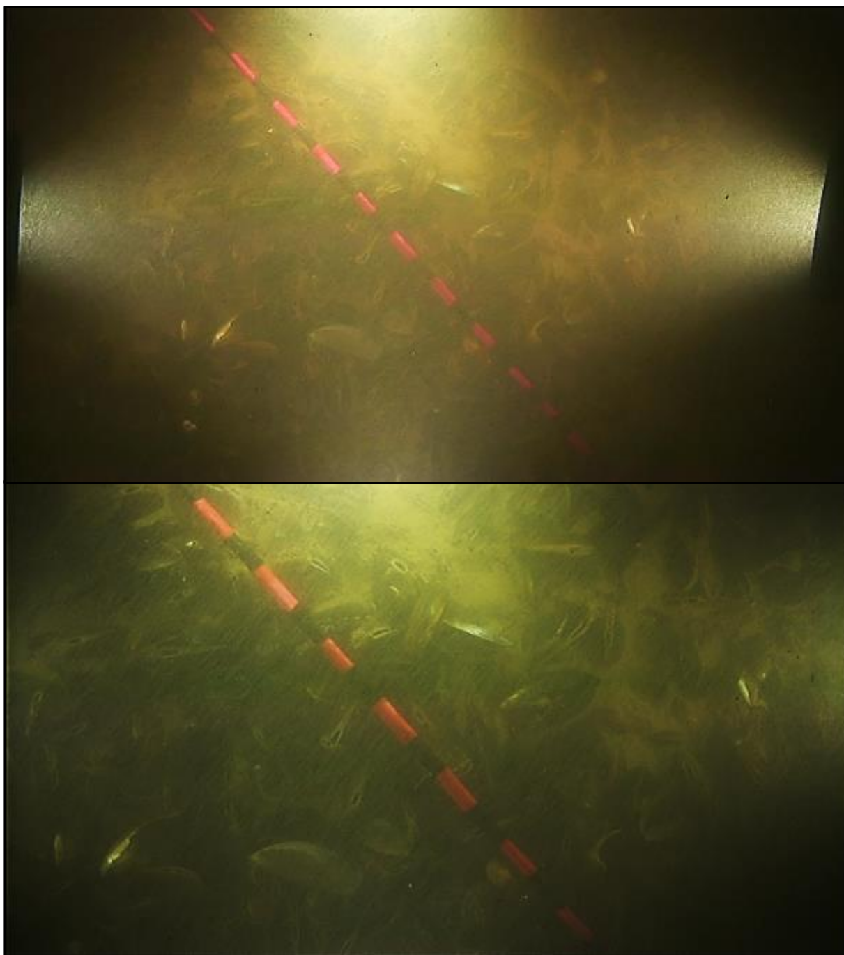
Figure 3.13: Screenshots of video footage captured at line STN_32 in the Solway Firth SAC survey area (sample 412_037#01_02) showing Mytilus edulis bed (top = full field of view; bottom = full zoom whilst camera landed. Scale bar in increments of 2 cm).
