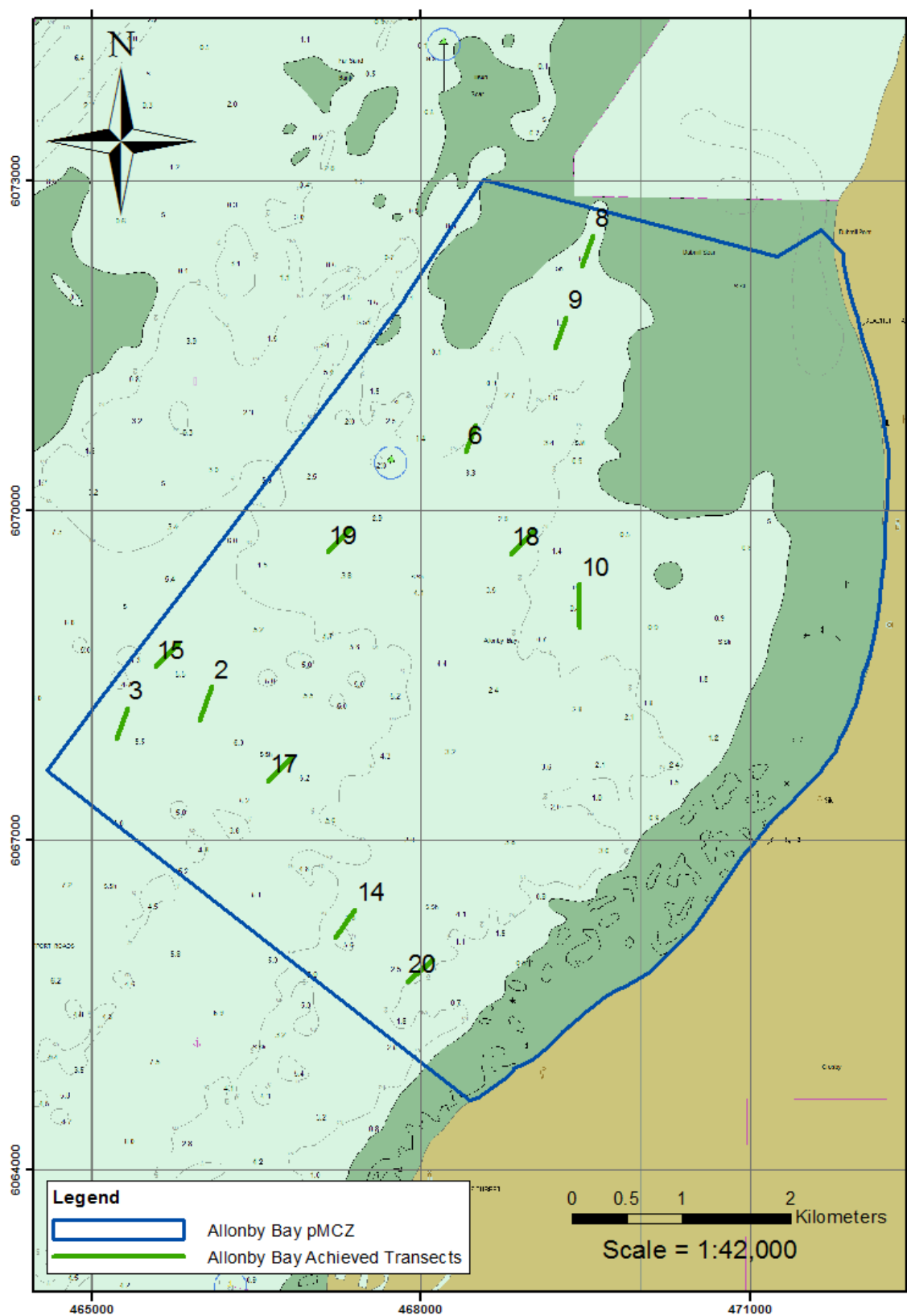
Figure 3.1: Achieved video camera transect locations within the Allonby Bay pMCZ
