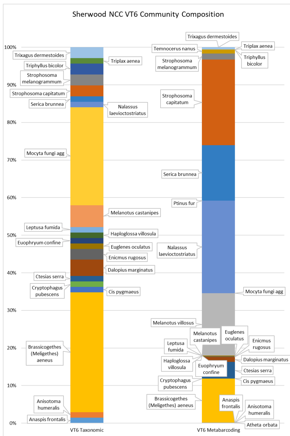
Figure 3.17 Community composition of Sherwood NCC sample VT6. Bar sizes are based on the percentage abundance of number of individuals (taxonomic) or the percentage of number of sequence reads matching those species (metabarcoding). ‘Taxonomic’ refers to those species that were hand identified and ‘metabarcoding’ refers to those species that were identified by metabarcoding. For all samples, those species that do not appear in the BOLD database and those which are not in the order of interest were removed from the overall species list prior to bar chart creation. All species that were effectively removed by being retained by Natural England were removed from the overall species list prior to bar chart creation.
