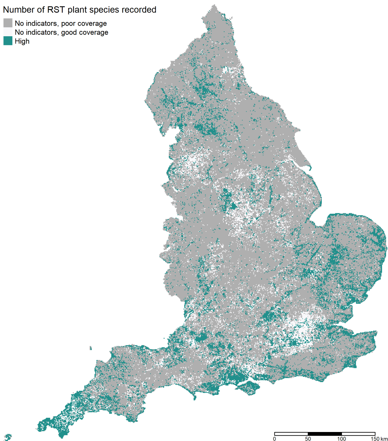
Figure 5: The distribution of Rare, Scarce and Threatened (RST) plant species at the monad scale (1 x 1 km grid cells) in England. 'High' represents monads with one or more RST species present; 'no indicators, good coverage' represents monads with good survey coverage, but no RST species recorded; "no indicators, poor coverage" indicates monads with poor survey coverage (<3 recording days) and no RST plant species recorded. © Copyright Natural England & Botanical Society of Britain and Ireland. Map attribution: Contains OS data © Crown copyright and database right 2021. Source: Office for National Statistics under Open Government Licence v.3.0.
