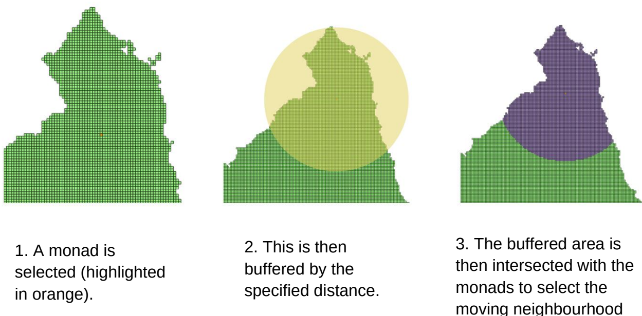
Figure 6: A diagram showing the process of selecting the moving neighbourhood of monads which is used to retrieve the species pool around a monad. Contains OS data © Crown copyright and database right 2021. Source: Office for National Statistics under Open Government Licence v.3.0.
