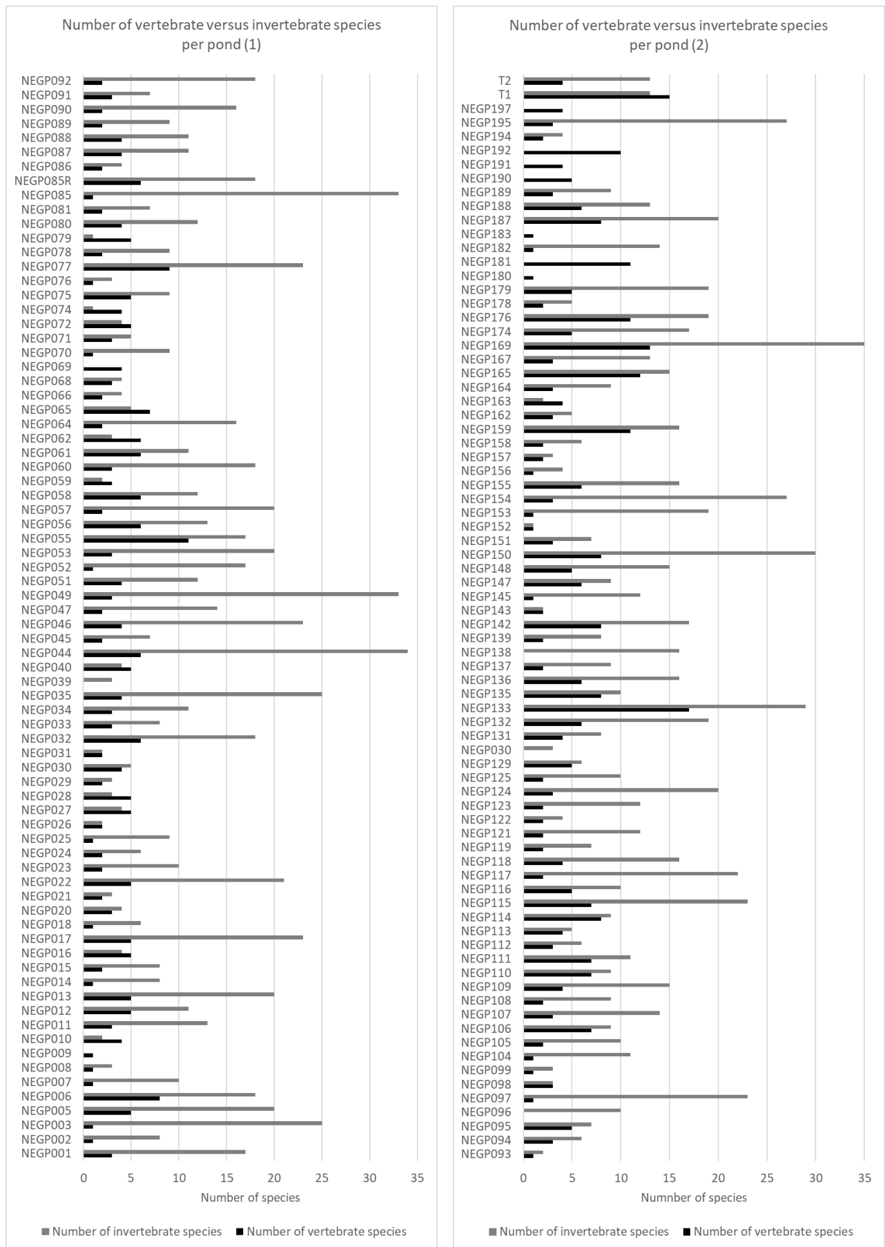
Figure 7. Comparison of the number of vertebrate and invertebrate species per pond.
