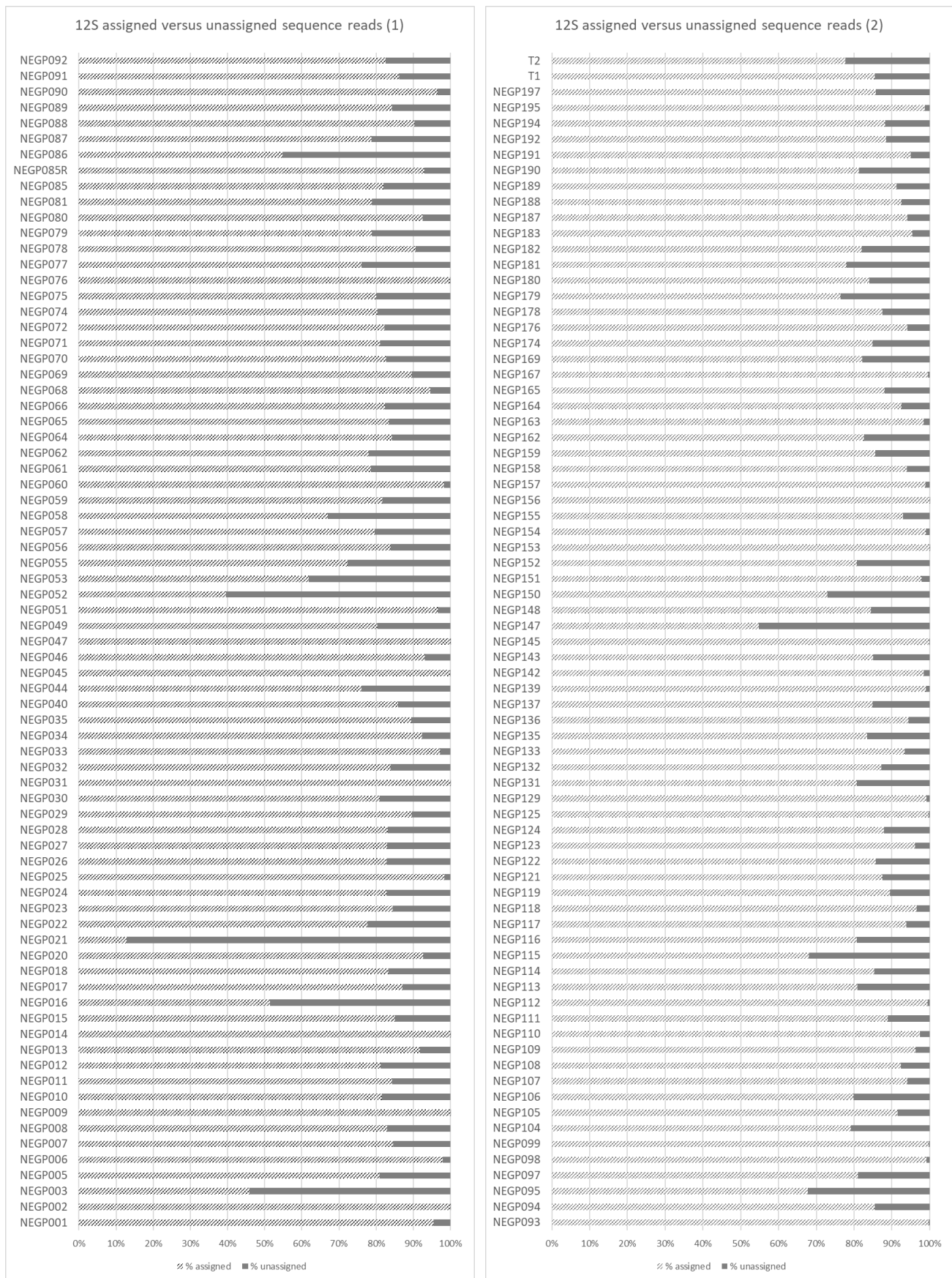
Figure 5 (1 and 2). 12S proportion of assigned and unassigned sequence reads.
